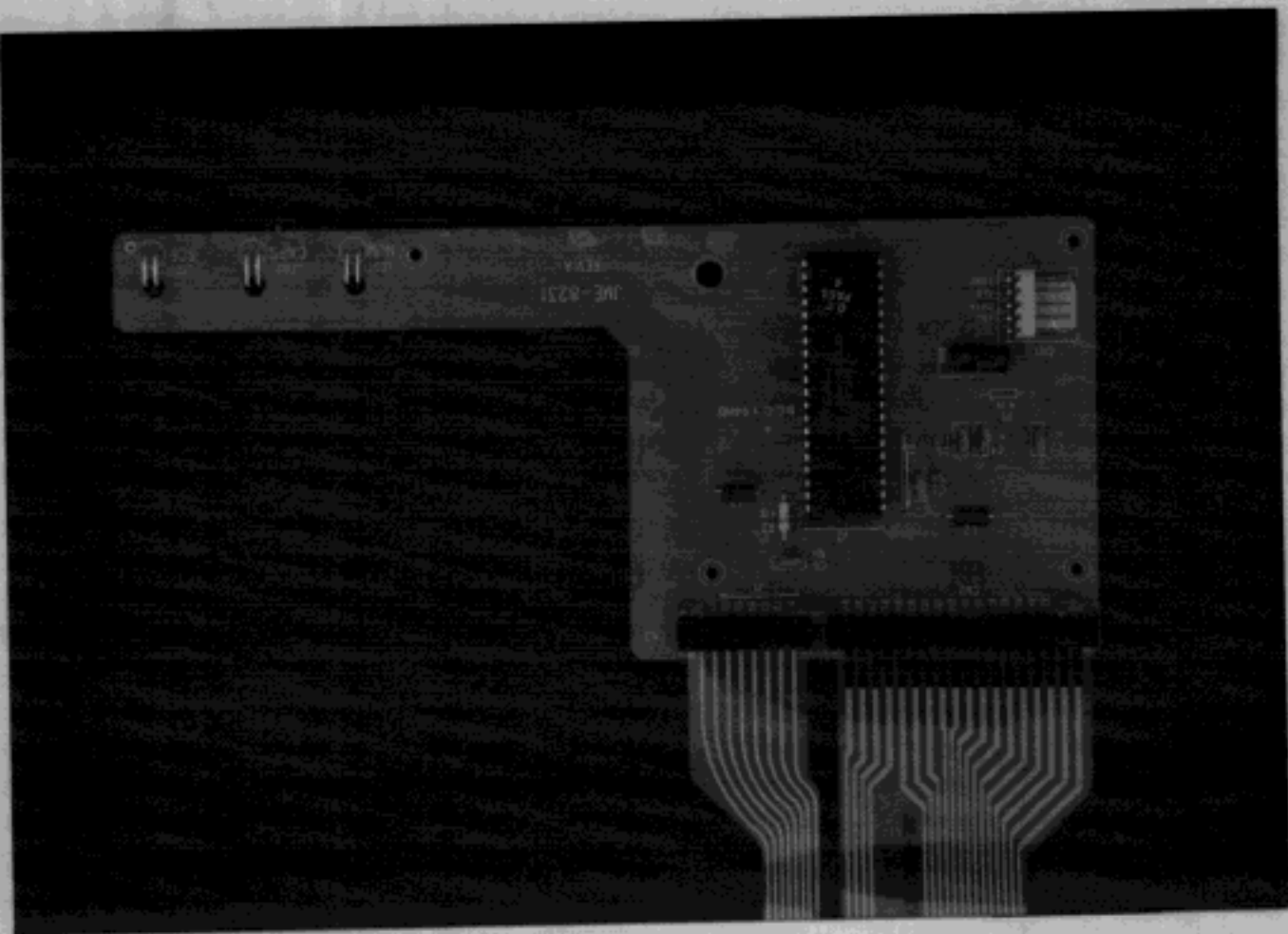
Figure 6 Main PCB Board, Component Side
