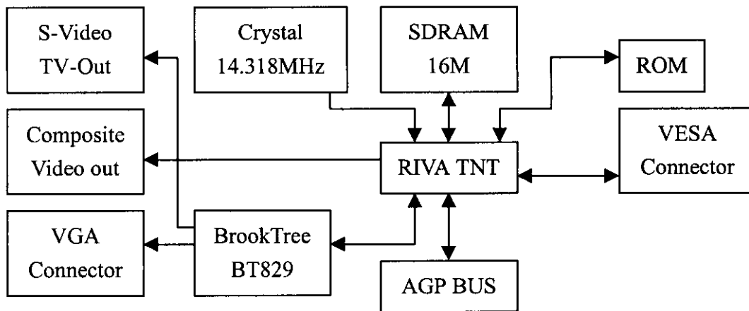
Apollo TNT Block Diagram
