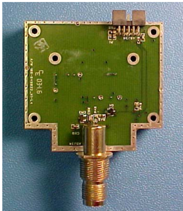
800 MHz Power Amp - Bottom View
