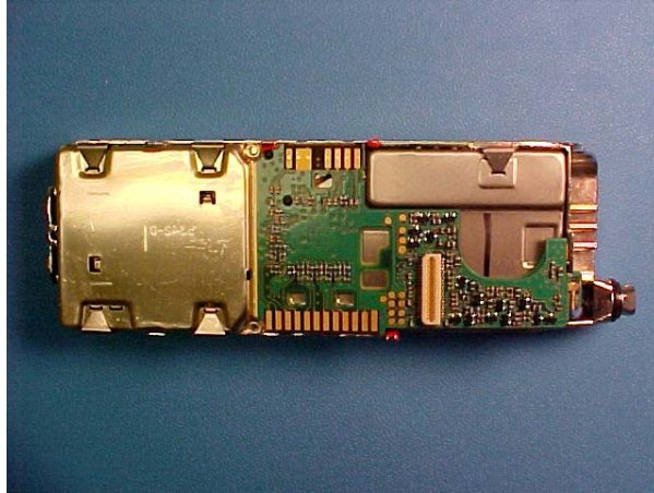
VHF Integrated Transceiver Module - Top View
