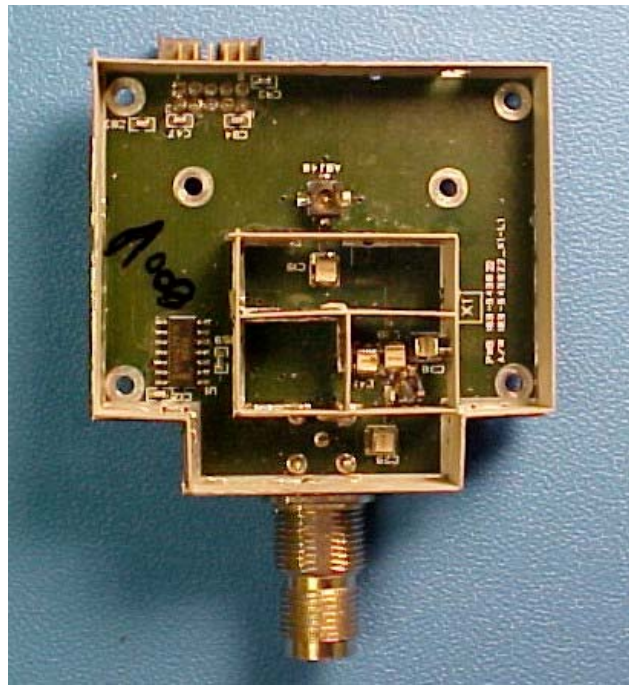
800 MHz Power Amp - Top View
