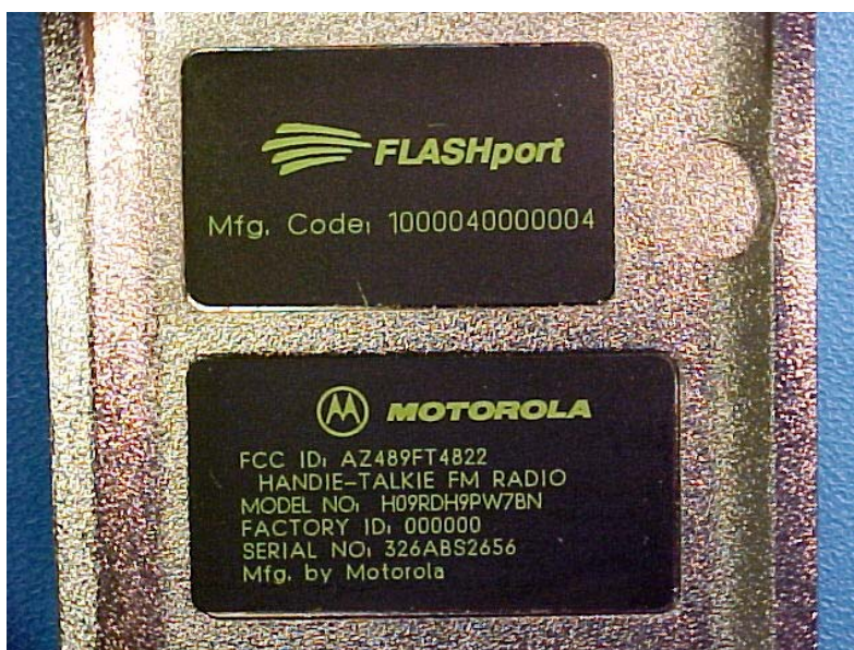
UHF-1 Integrated Transceiver Module: FCC ID- AZ489FT4822
