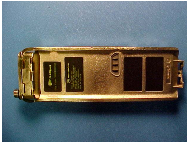
VHF Integrated Transceiver Module - Bottom View
