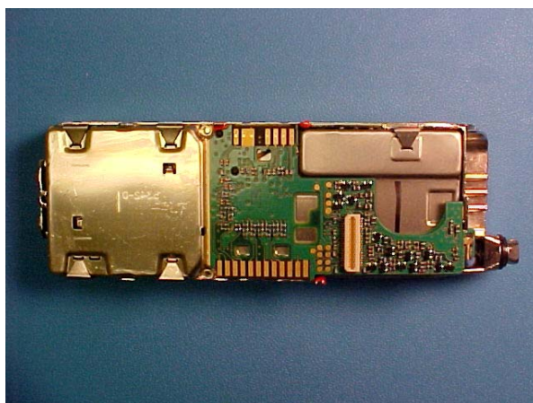
UHF-1 Integrated Transceiver Module - Top View
