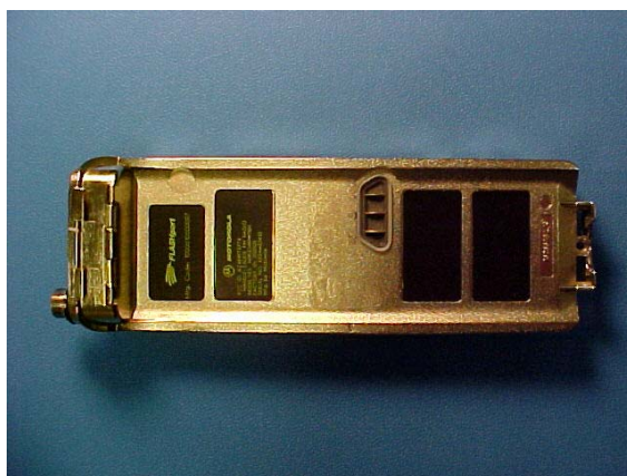
UHF-1 Integrated Transceiver Module - Bottom View
