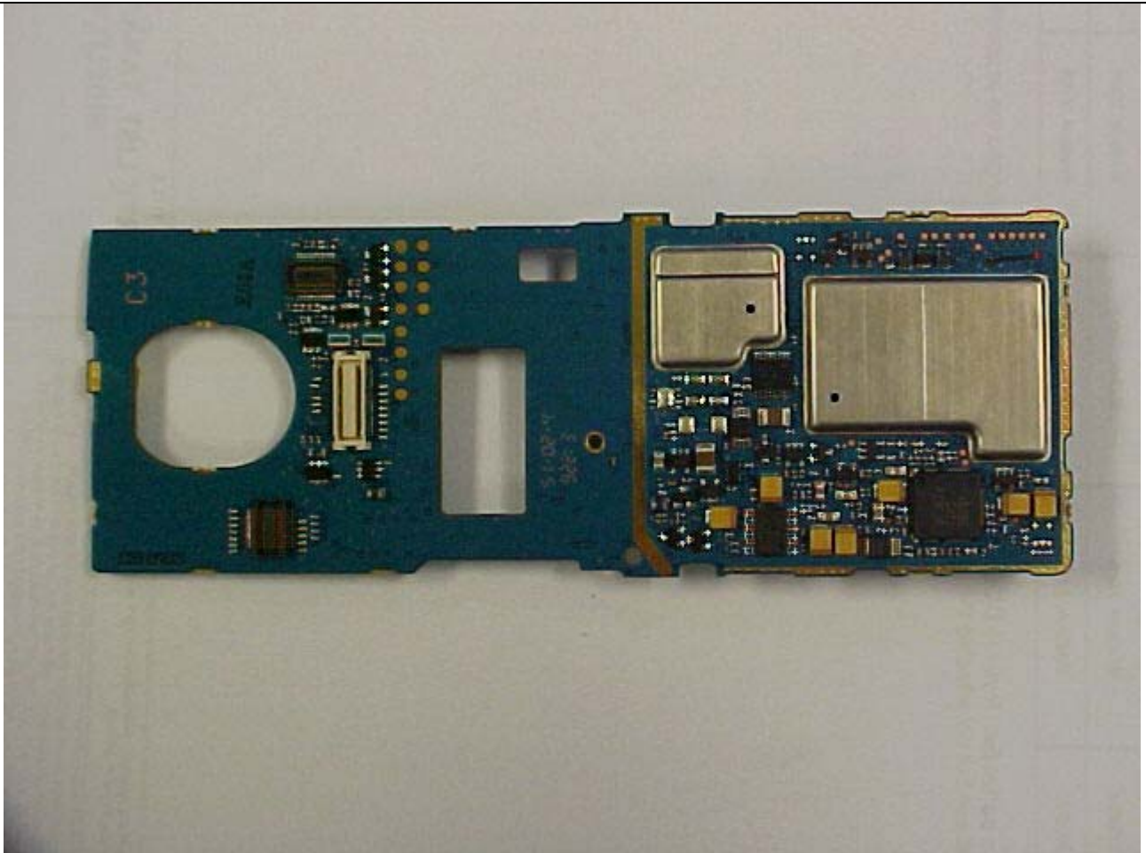
800 MHz Integrated Transceiver Module – Vocon Board Top View
