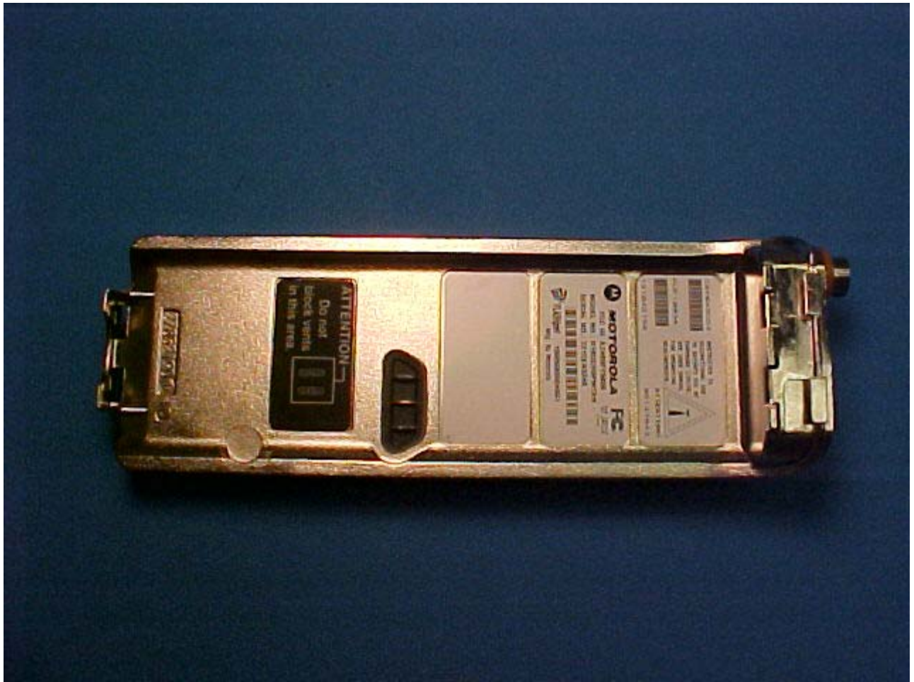
800 MHz Integrated Transceiver Module - Bottom View
