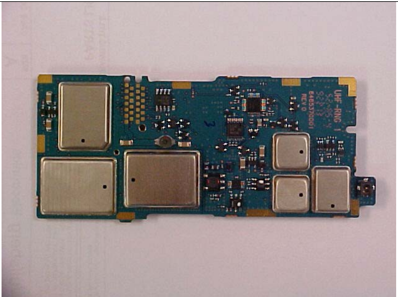
UHF1A Integrated Transceiver Module – Transceiver Board Top View
