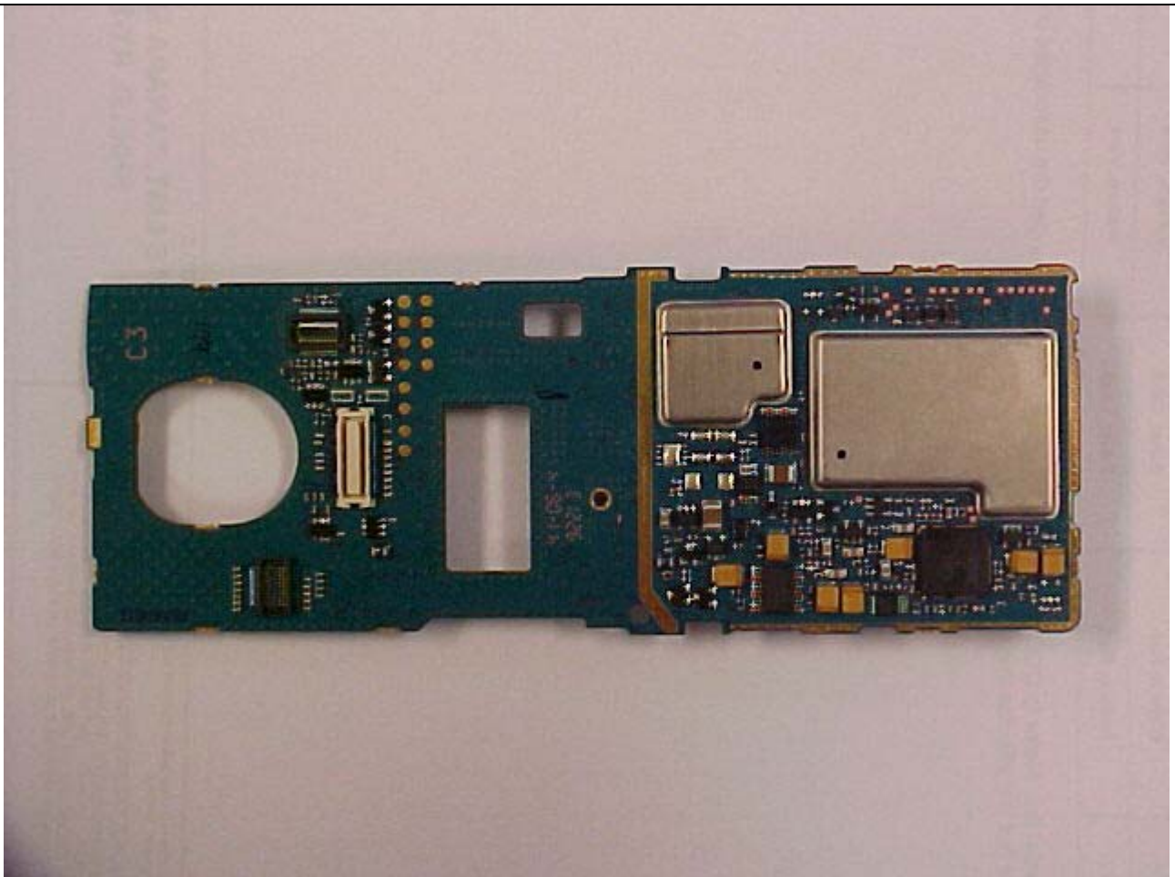
UHF1A Integrated Transceiver Module – Vocon Board Top View
