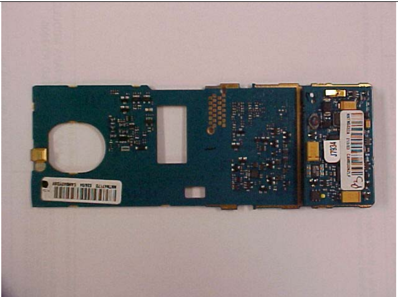
UHF1A Integrated Transceiver Module – Vocon Board Bottom View
