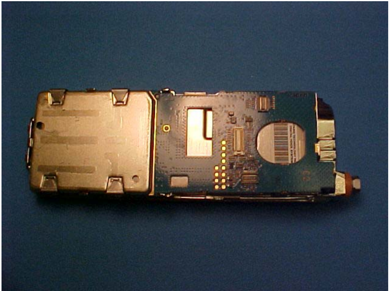
UHF2A Integrated Transceiver Module - Top View
