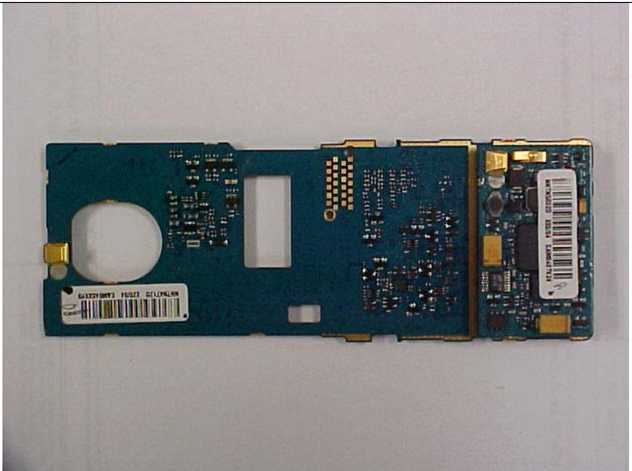
UHF2A Integrated Transceiver Module – Vocon Board Bottom View
