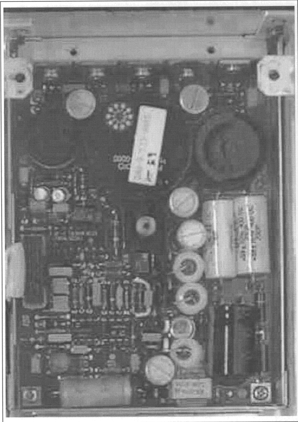
Figure 4: VC-401 Power Supply
