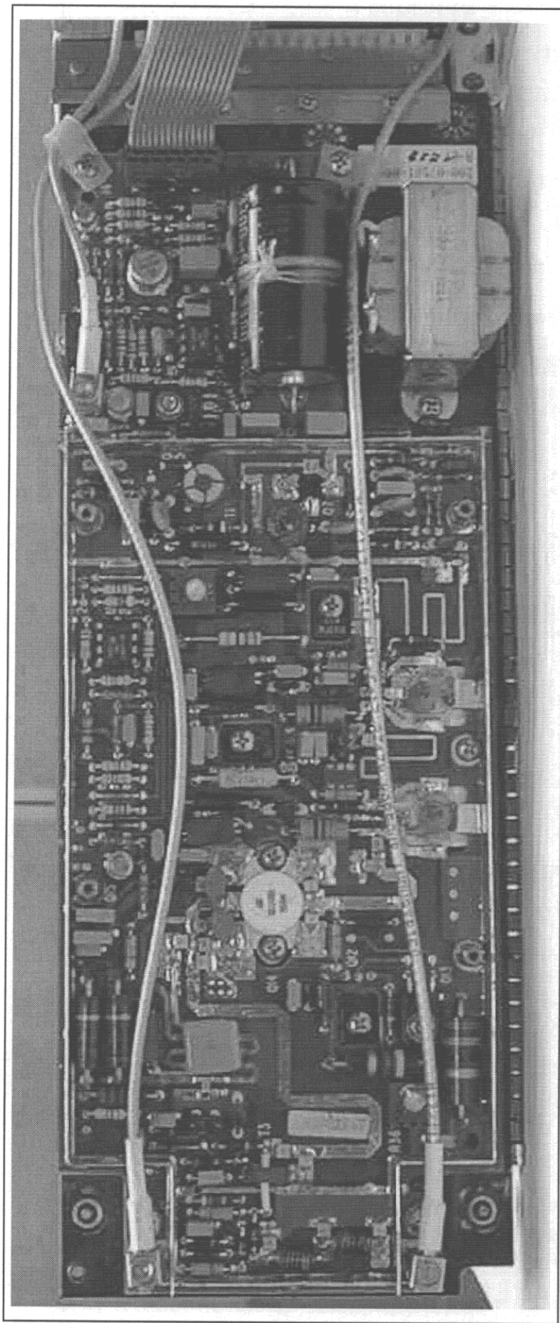
Figure 6: VC-401 Transmitter Module
