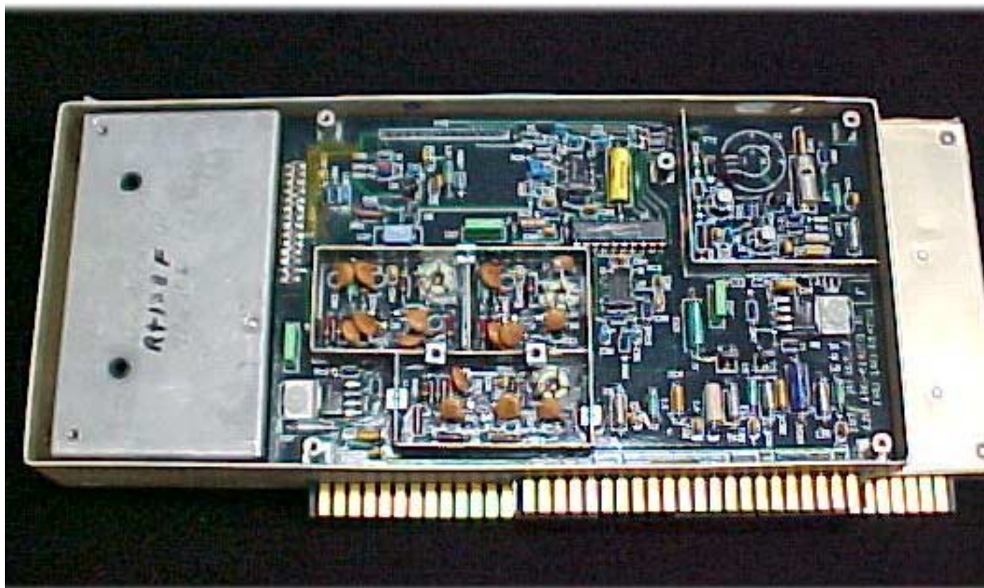
Internal Photos Synthesizer Board
