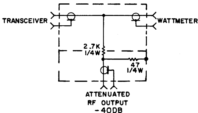
R.F. ISOLATION PAD SCHEMATIC FIGURE 2.2-1
