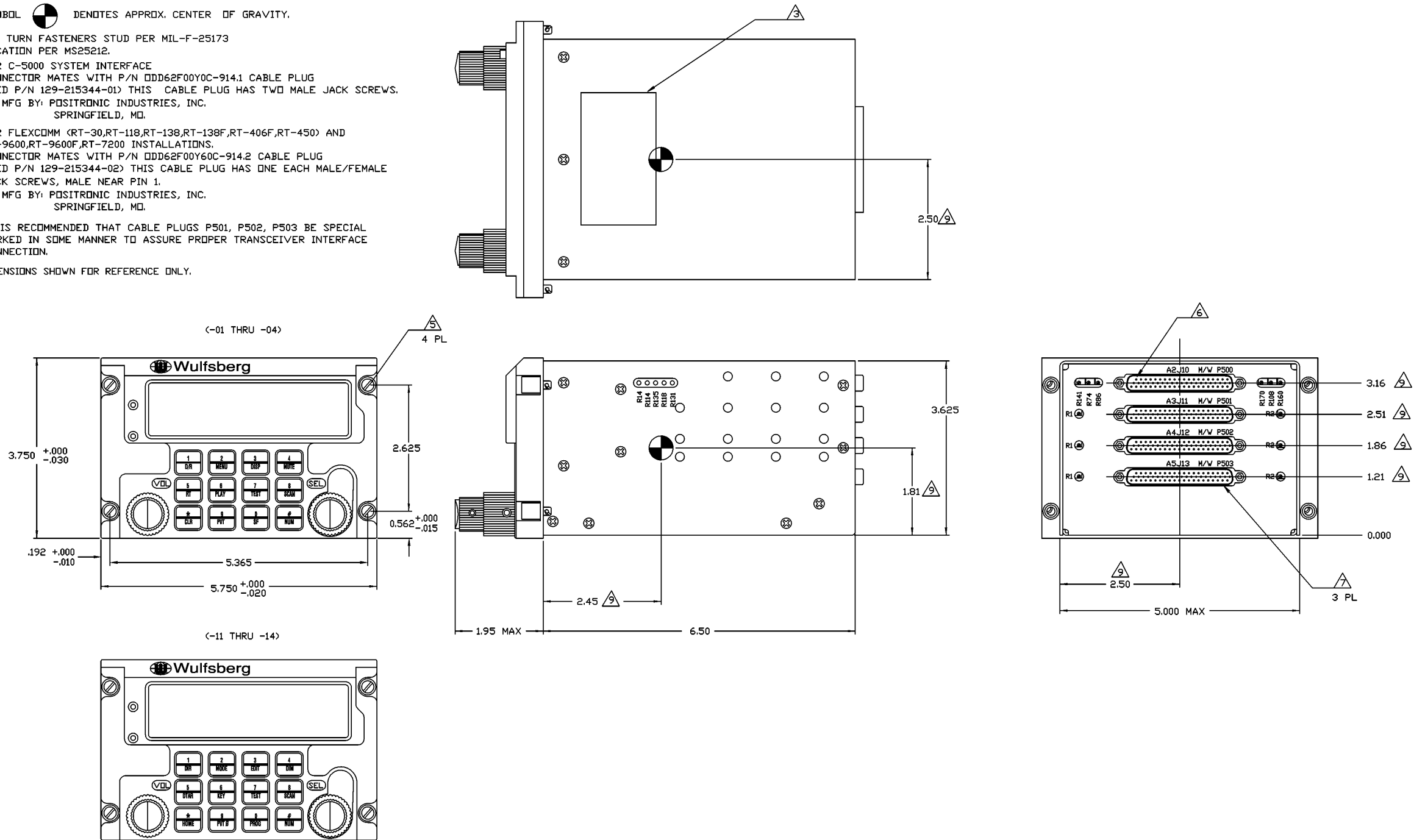
Figure 3-1. C-5000 Envelope Drawing (Sheet 1 of 1) Dwg No. 154-031300, Rev. F
