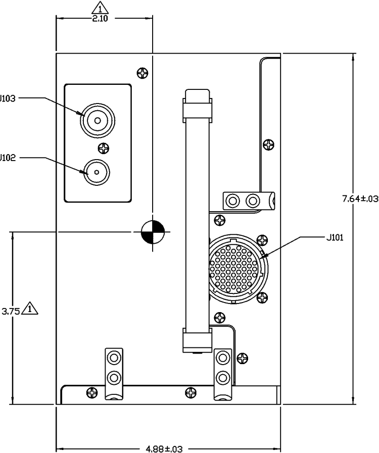
Figure 3-2. RT-5000 Envelope Drawing (Sheet 1 of 1) Dwg No.154-015525, Rev D
