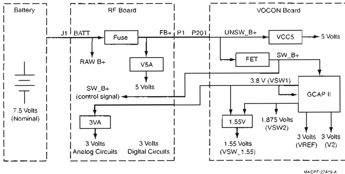
Figure 2-1. DC Power Distribution—UHF Range 1 and 700–800 MHz Radios
