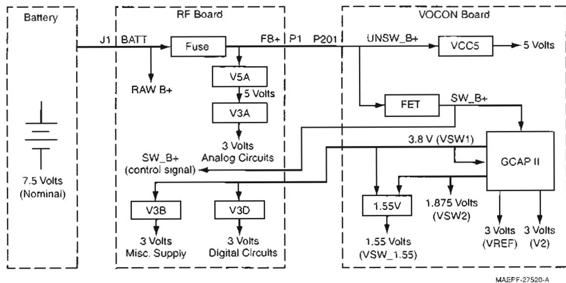
Figure 2-2. DC Power Distribution—VHF and Range 2 Radios
