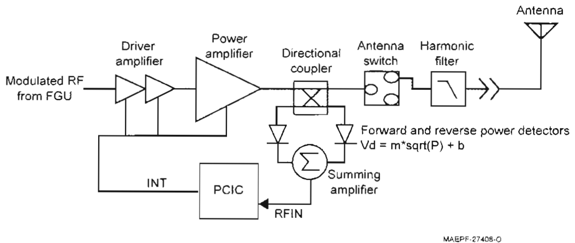
Figure 3-6. Transmitter Block Diagram
