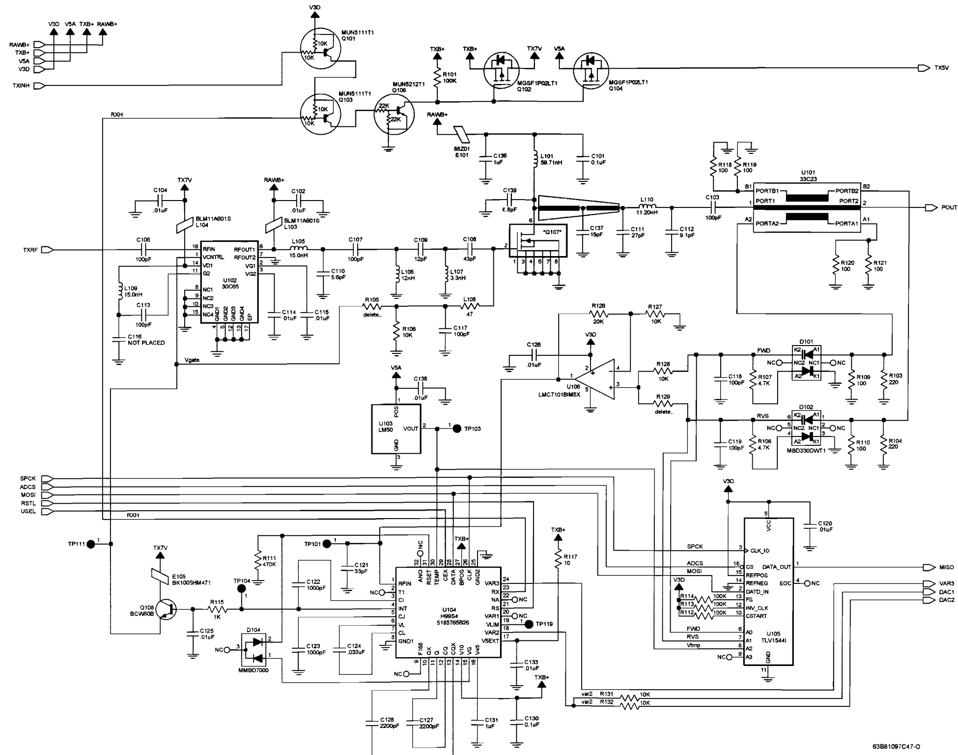
Figure 8-44. NLE4278A UHF Range 1 Transmitter Power Amplifier and Automatic Level Control Circuit
