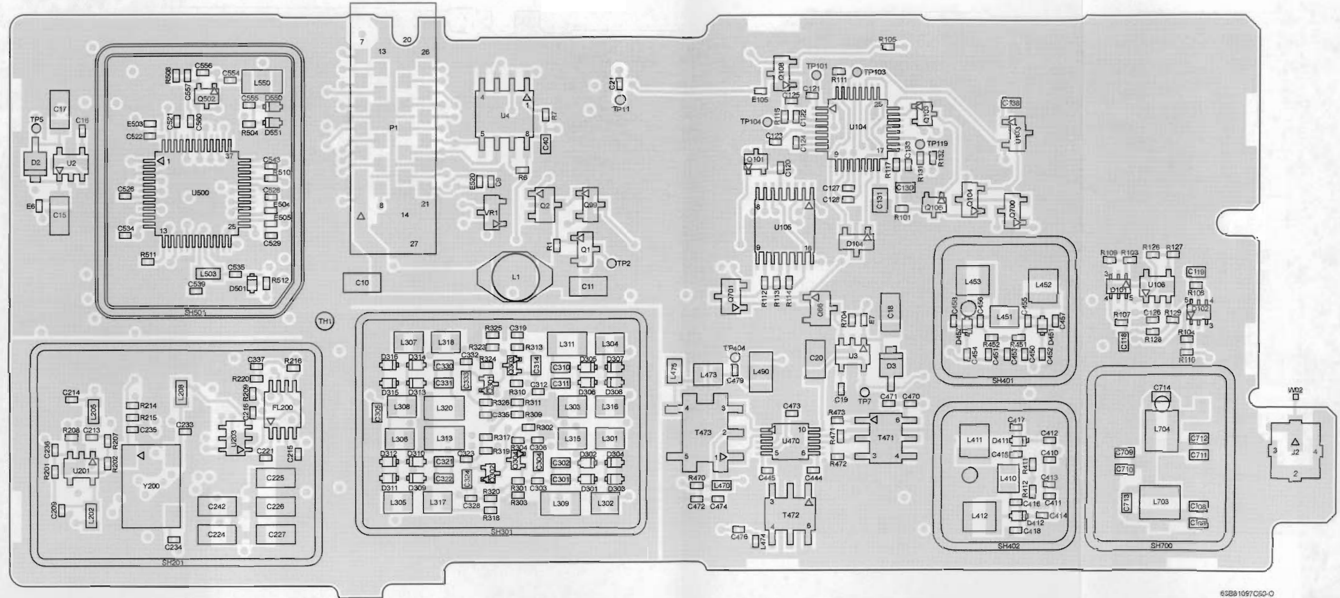
Figure 8-47. NLE4278A UHF Range 1 Transceiver (RF) Board Layout—Side 1
