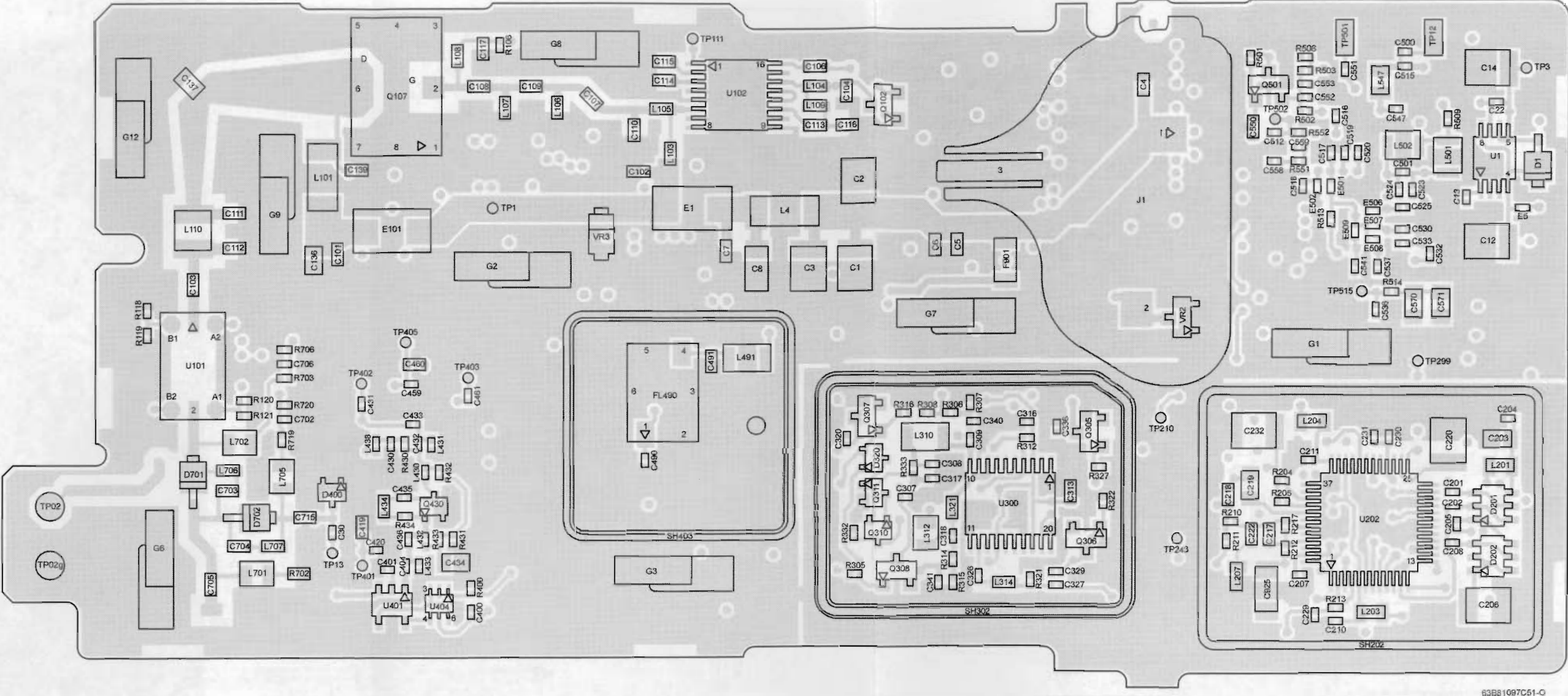
Figure 8-48. NLE4278A UHF Range 1 Transceiver (RF) Board Layout—Side 2
