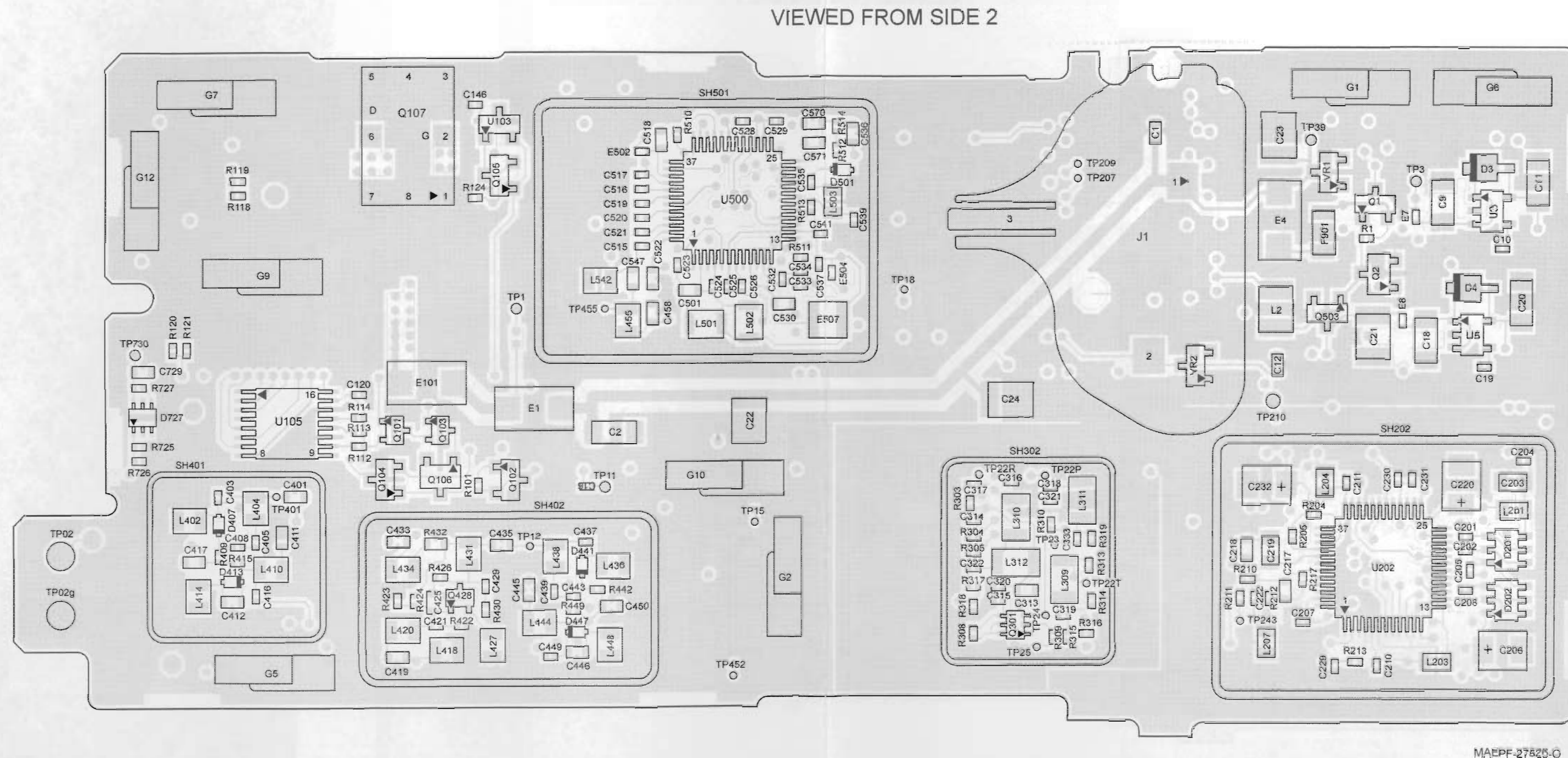
Figure 8-30. NLD8910B VHF Transceiver (RF) Board Layout—Side 2
