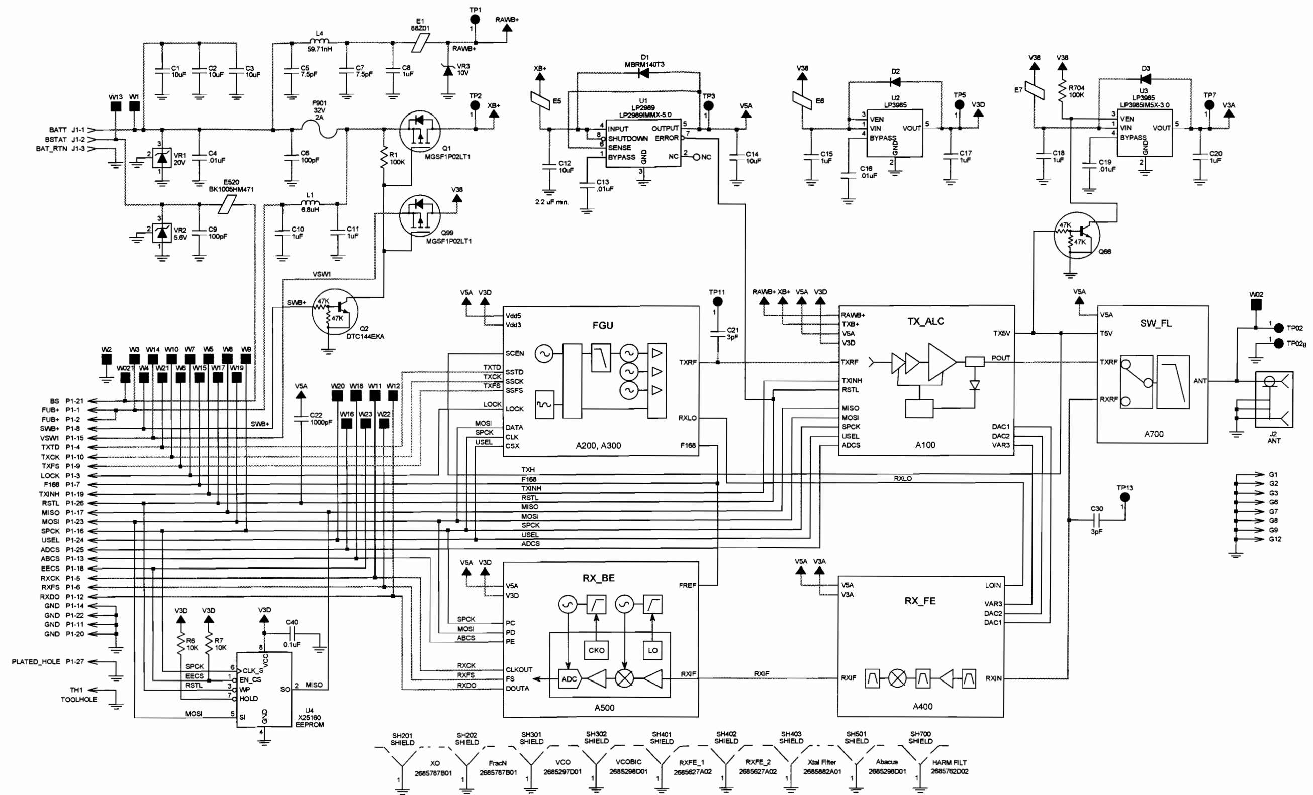
Figure 8-31. NLE4272A UHF Range 1 Transceiver (RF) Board Overall Circuit Schematic
