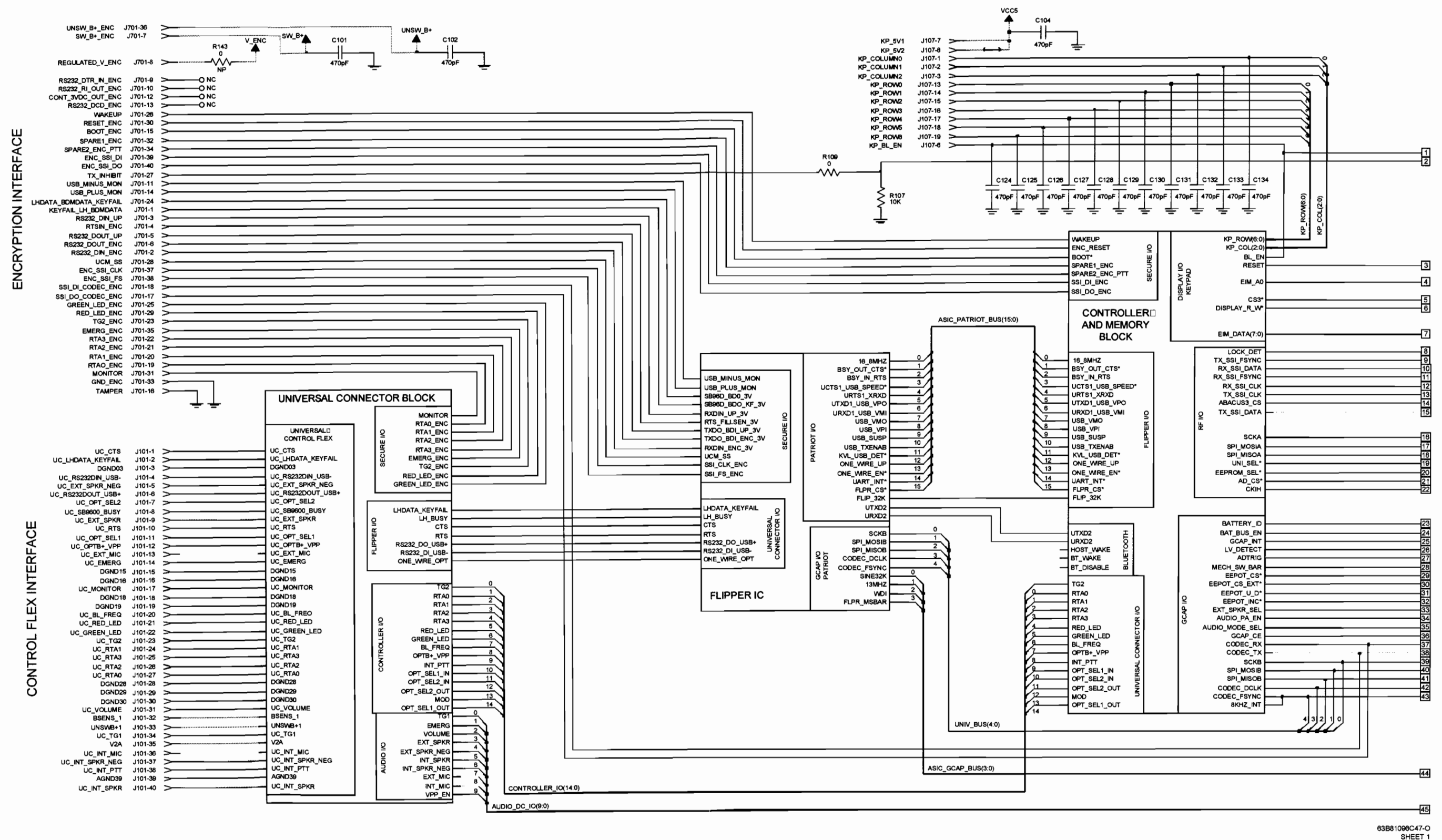
Figure 8-70. NTN9564C VOCON Board Overall Schematic—1 of 2
