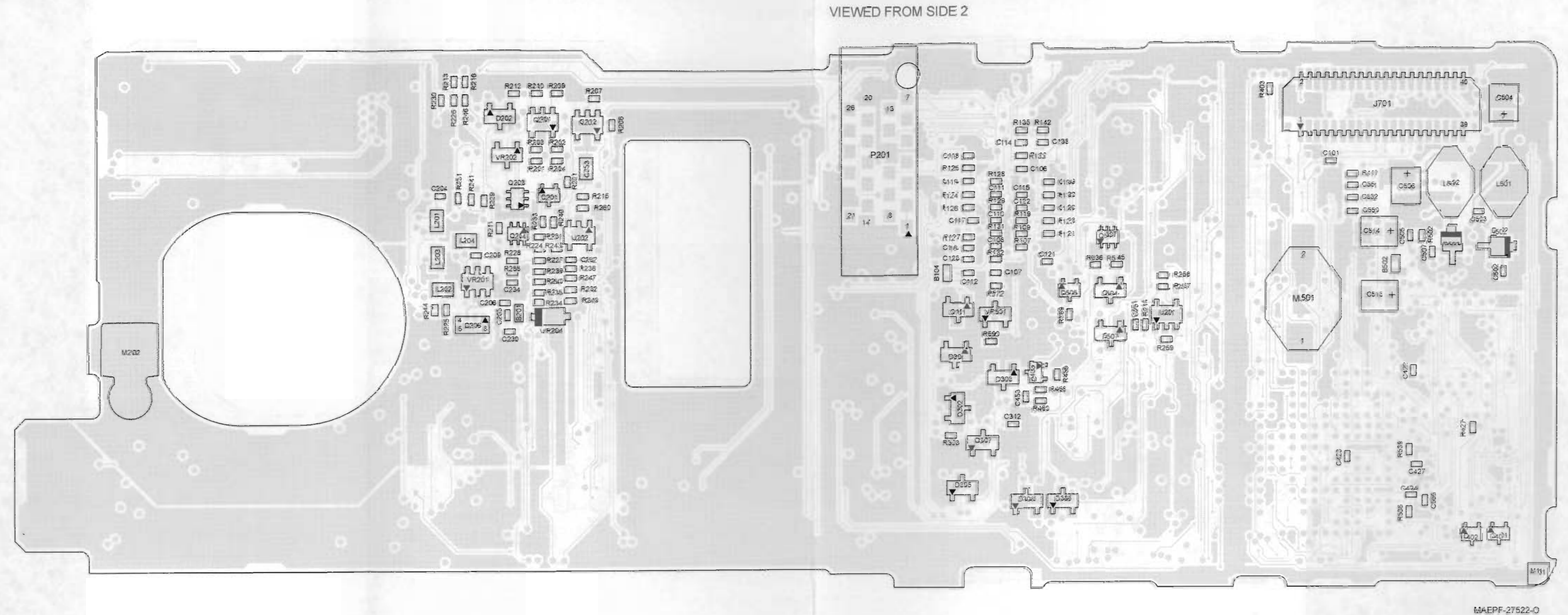
Figure 8-78. NTN9564C VOCON Board Layout—Side 2
