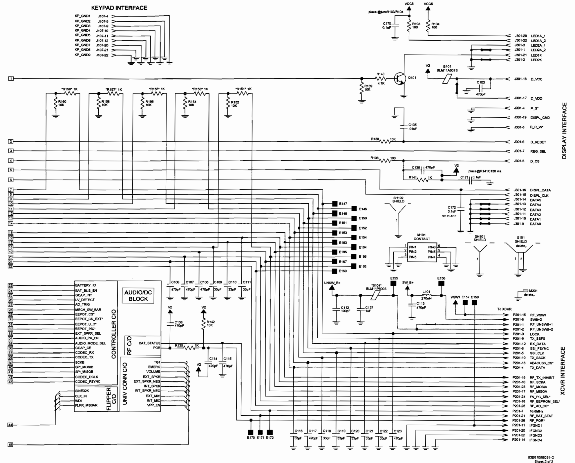
Figure 8-89. NNTN4819A VOCON Board Overall Schematic—Sheet 2 of 2
