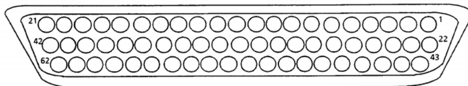
Figure 4-14. Connector P501/P502
