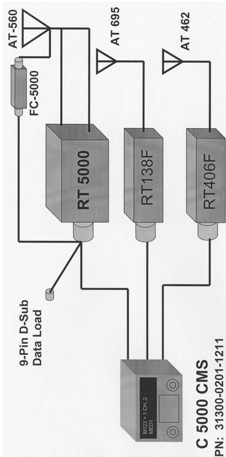
Figure B-2. Configuration #1 (Basic RT-5000)
