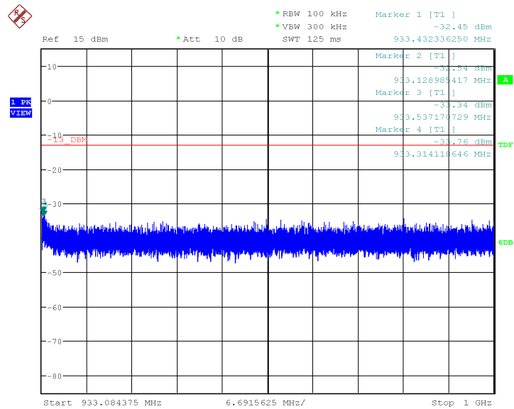
spur_8k10f1e_932.00625_30m1g_high.png
