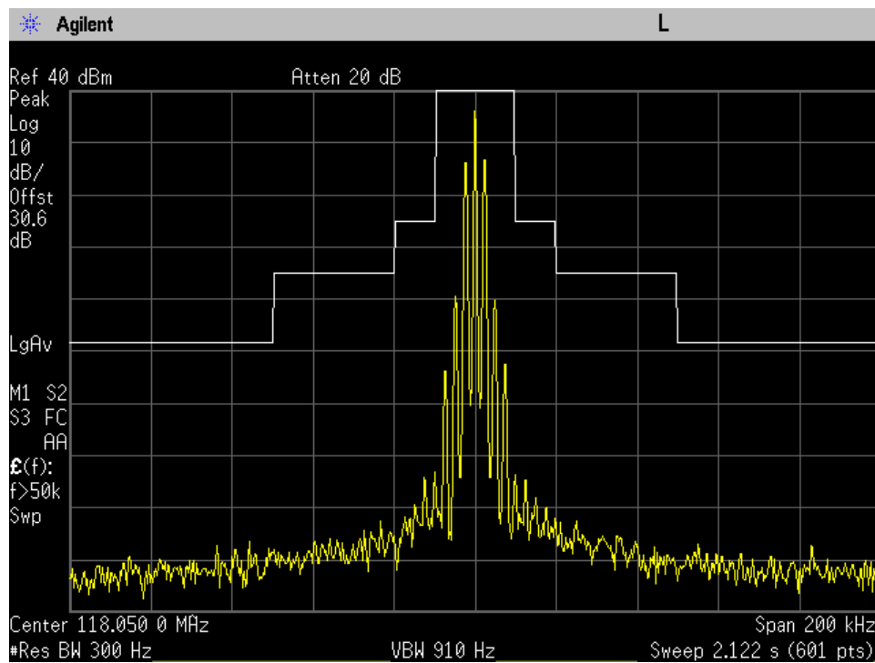
118.05_25K_Mask B
