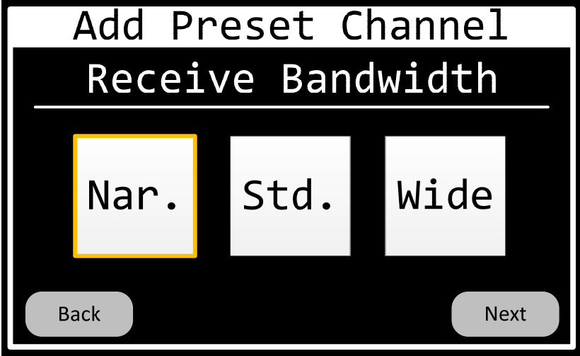
Figure 65 Preset-Channel-Receive-Bandwidth Page
