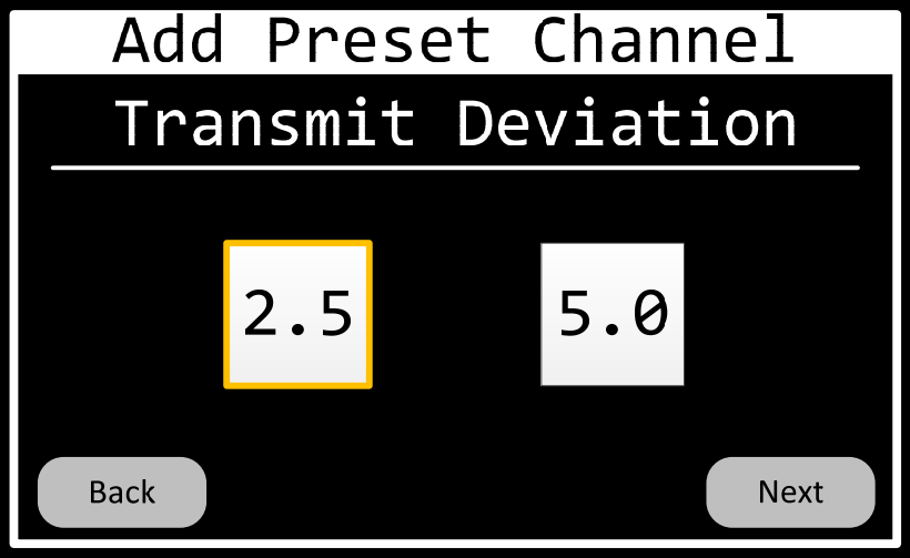
Figure 64 Preset-Channel-Transmit-Deviation Page
