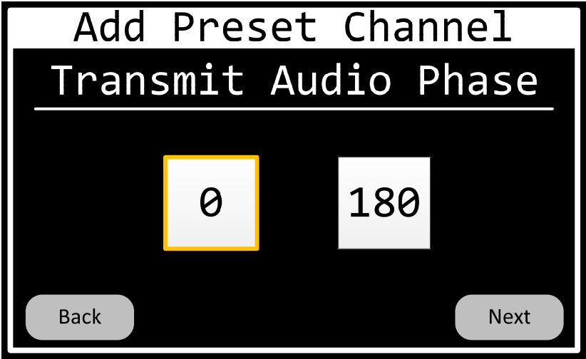
Figure 63 Preset-Channel-Transmit-Phase Page
