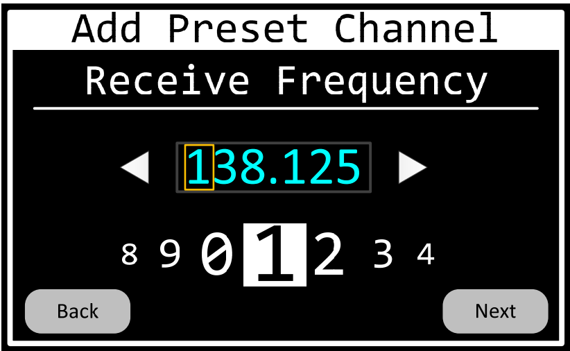
Figure 52 Preset-Channel-Receive-Frequency Page
