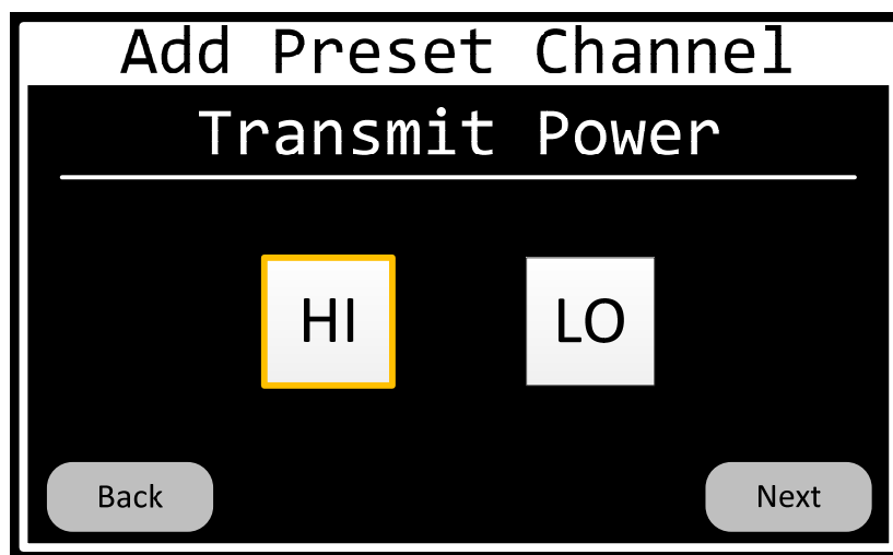
Figure 58 Preset-Channel-Transmit-Power Page
