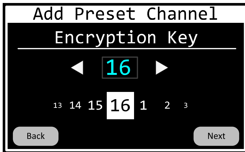
Figure 61 Preset-Channel-Encryption-Key Page
