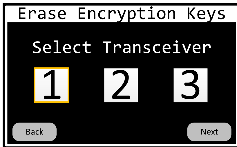
Figure 87 Encryption-Key-Erase-Transceiver Page
