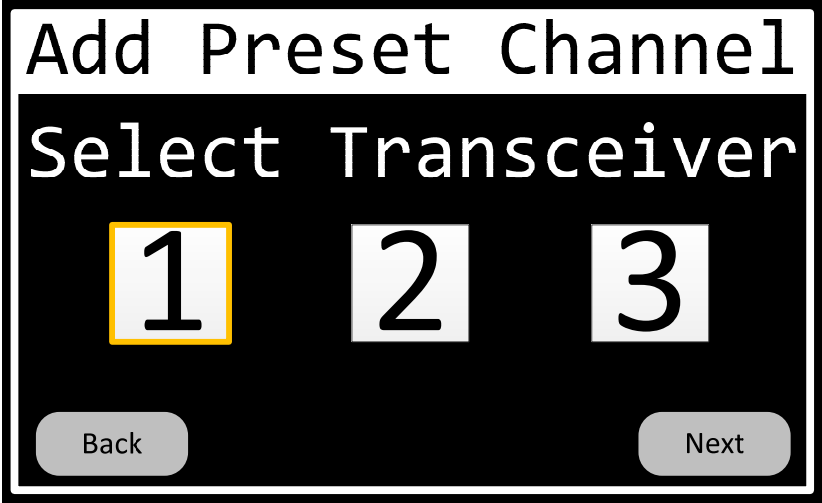
Figure 48 Preset-Channel-Transceiver Page
