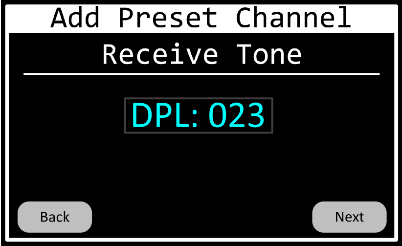
Figure 53 Preset-Channel-Receive-Tone Page
