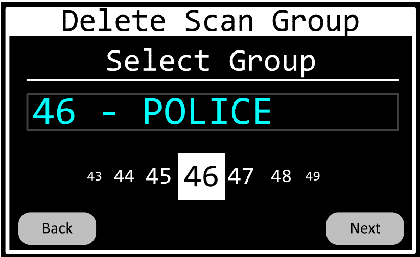
Figure 82 Scan-Group-Delete-Number Page
