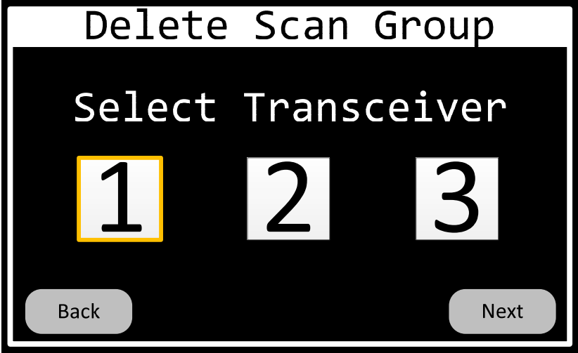
Figure 81 Scan-Group-Delete-Transceiver Page
