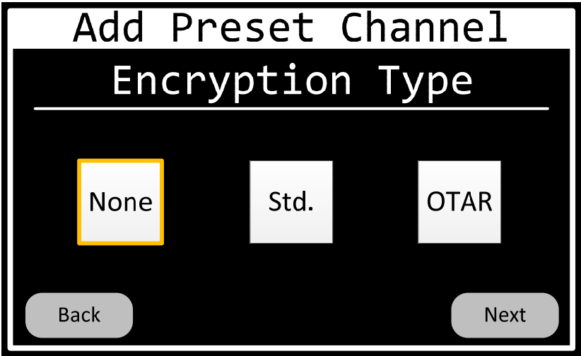
Figure 60 Preset-Channel-Encryption-Type Page
