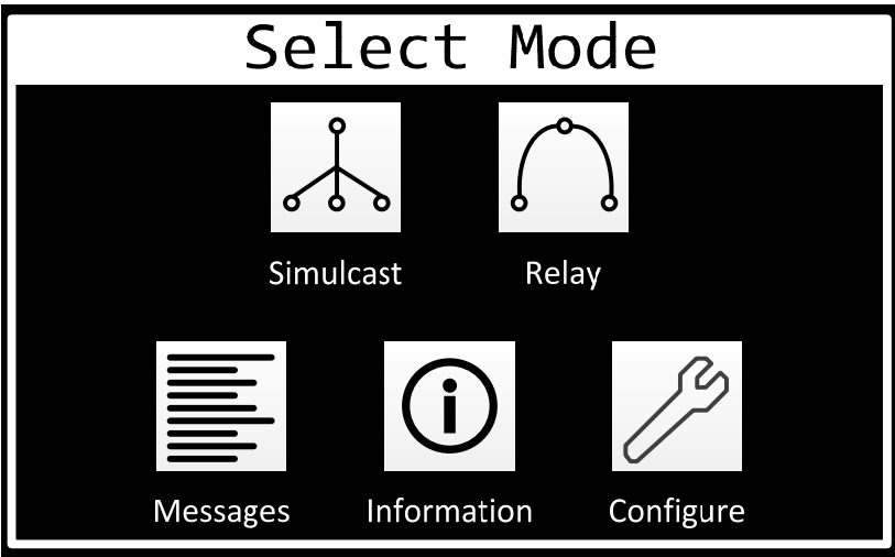
Figure 36 Mode-Selection-Menu Dialog
