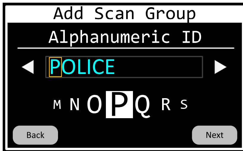
Figure 77 Scan-Group-Add-Alpha Page
