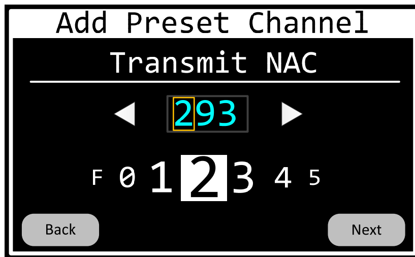
Figure 57 Preset-Channel-Transmit-NAC Page
