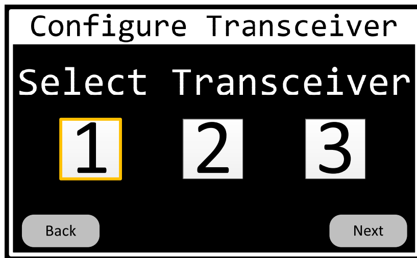
Figure 89 System-Configuration-Xcvr-Transceiver Page
