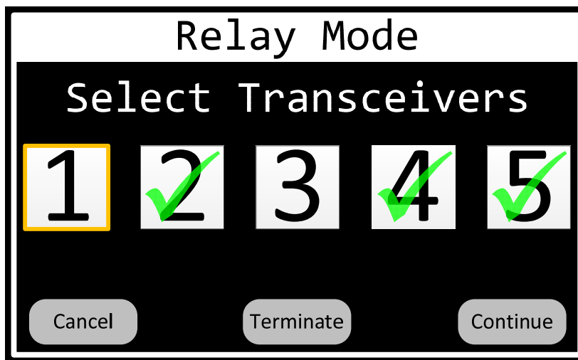
Figure 37 Relay-Configuration Dialog
