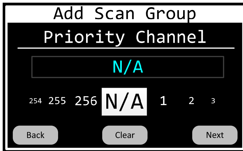
Figure 79 Scan-Group-Add-Priority-Channel Page
