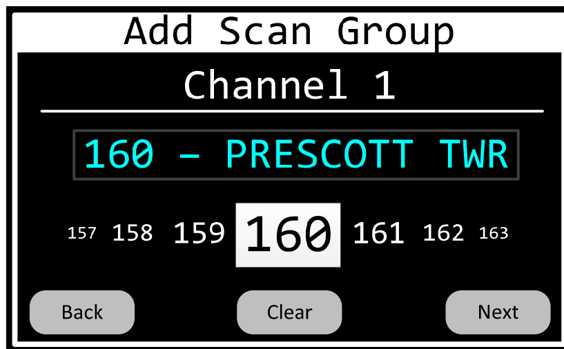
Figure 78 Scan-Group-Add-Channel-1 Page
