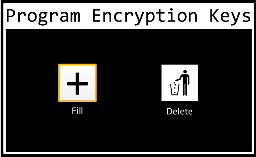
Figure 84 Encryption-Key-Function Dialog
