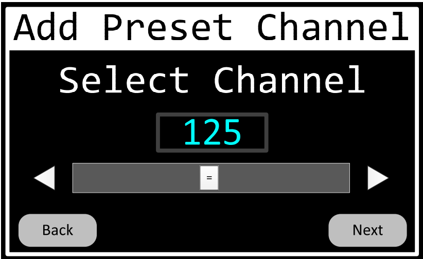
Figure 49 Preset-Channel-Number Page
