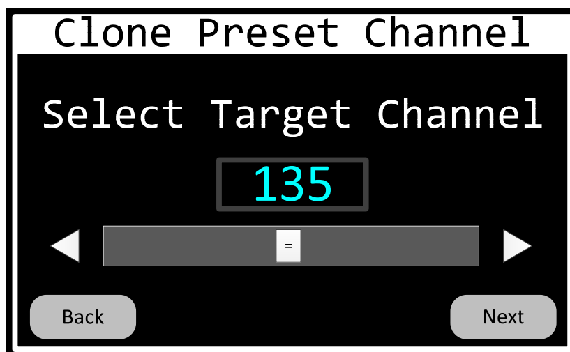
Figure 72 Clone-Preset-Channel-Target Page
