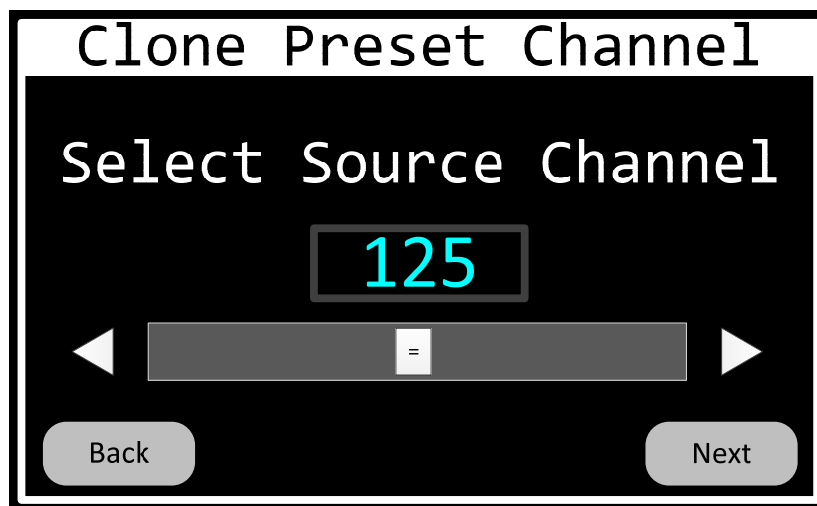
Figure 71 Clone-Preset-Channel-Source Page
