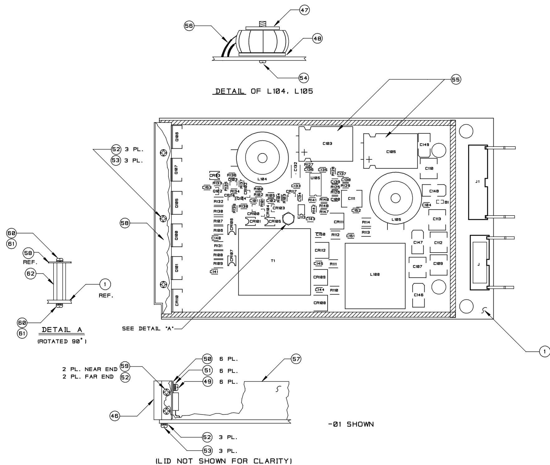
Figure 5-4. VC-401B VC-401B (8.33 kHz) Power Supply Module Parts Locator
