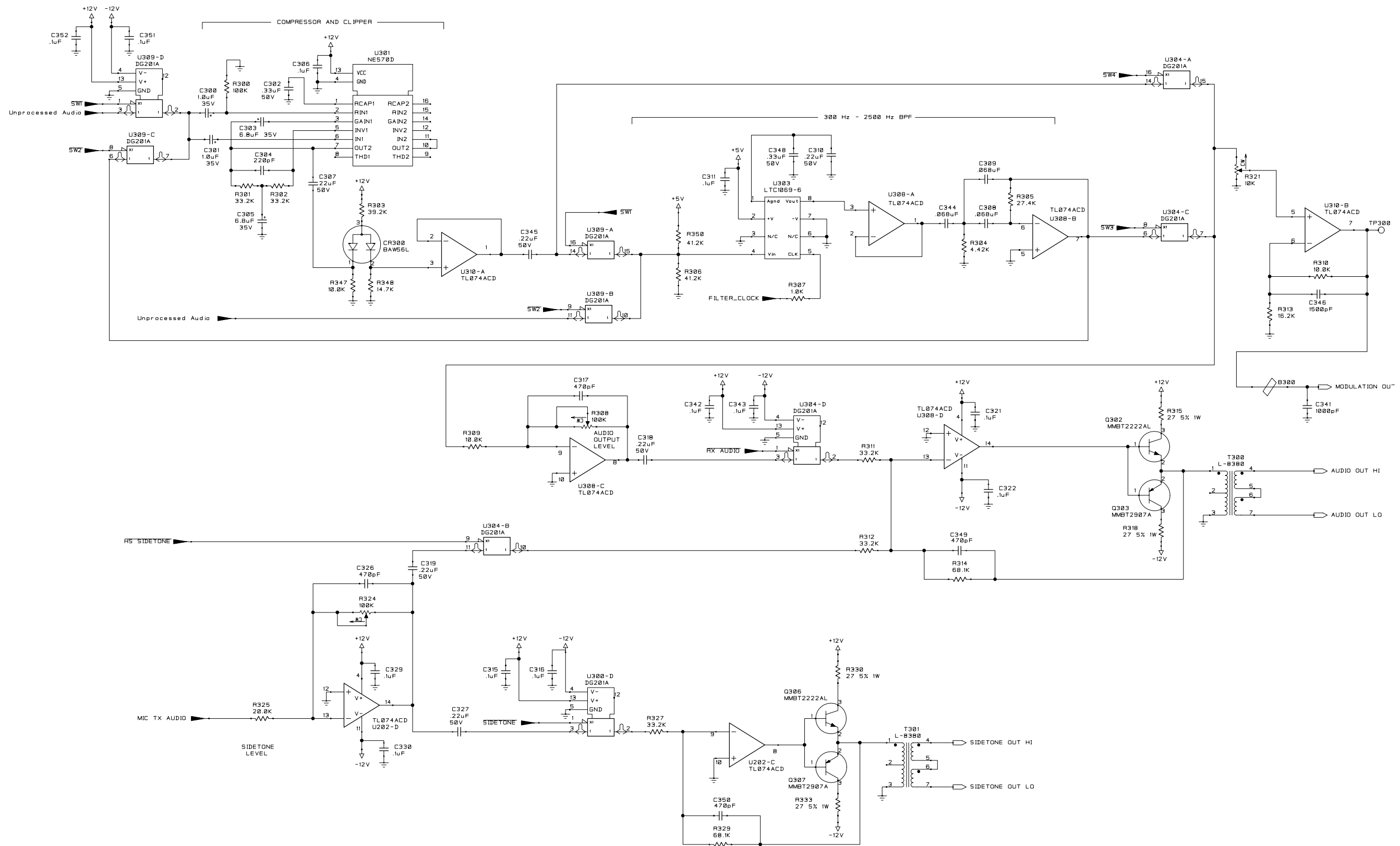
Figure 4-7. VC-401B VHF Communications Transceiver Audio/CPU Module Schematic Drawing (3 of 4)
