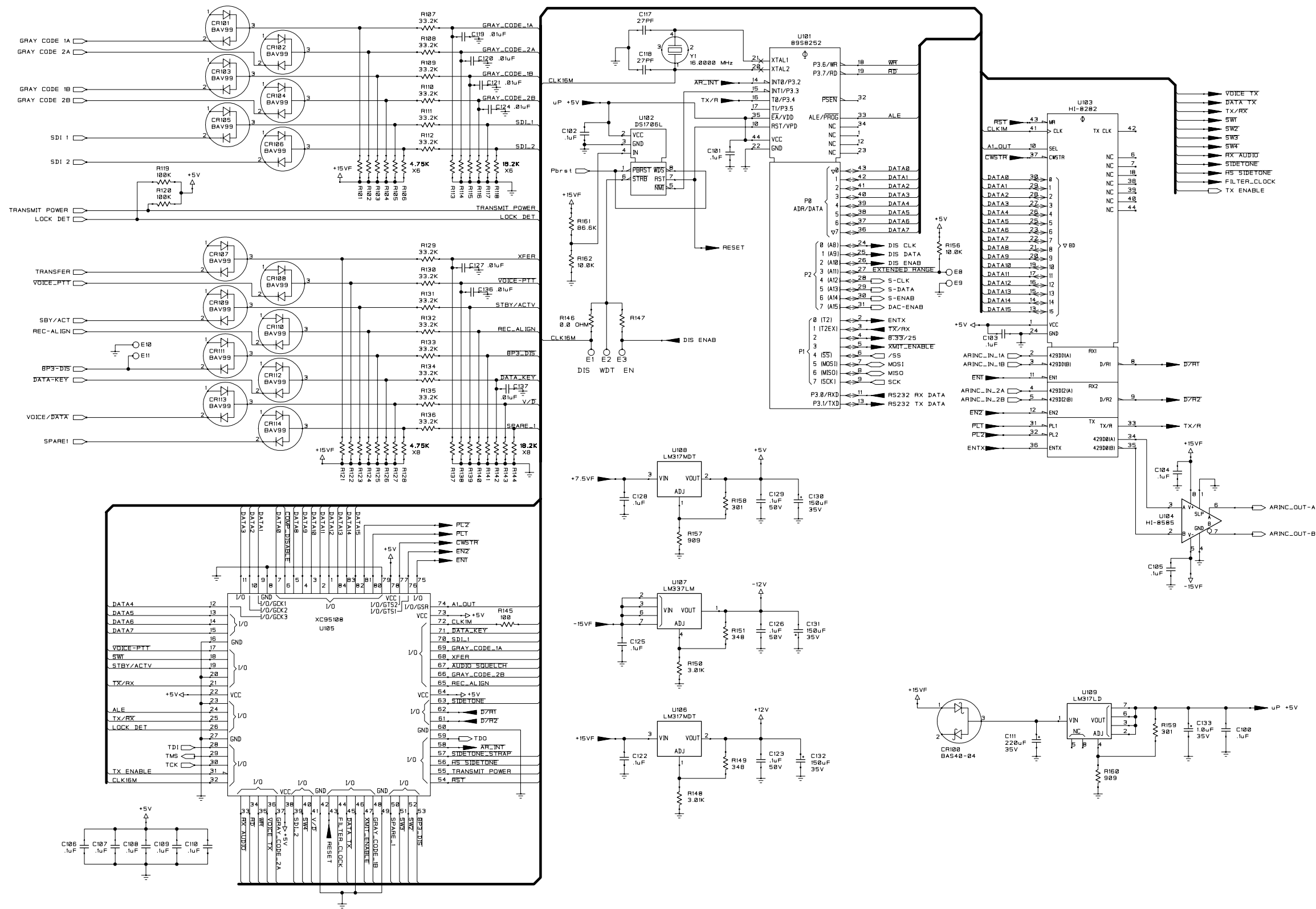
Figure 4-5. VC-401B VHF Communications Transceiver Audio/CPU Module Schematic Drawing (1 of 4)
