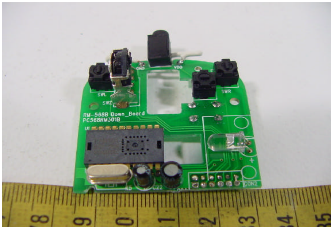
Component View of PCB
