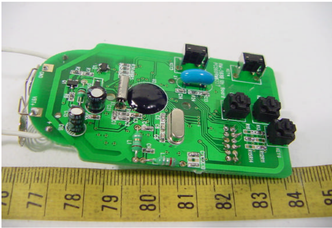
Component View of Main PCB
