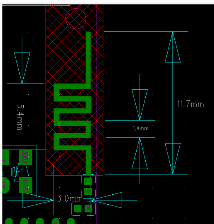
AntennaPhoto&Length (mm)
