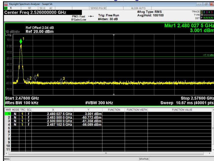
GFSK: Band Edge, Right Side
