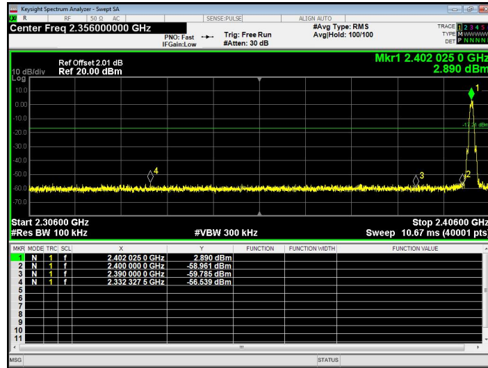
GFSK: Band Edge, Left Side
