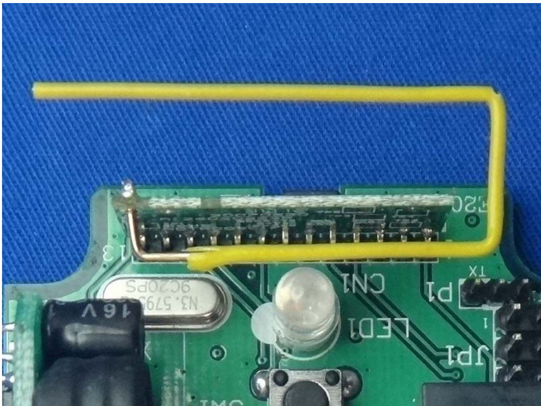
(11) EUT Photo-Antenna
