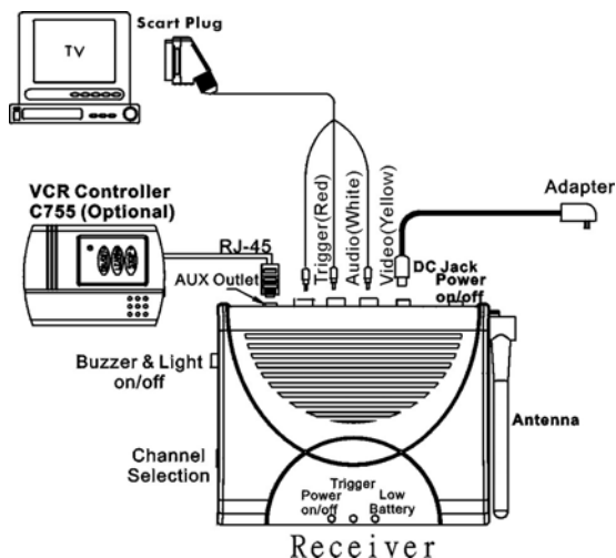
Figure 6 European Version
