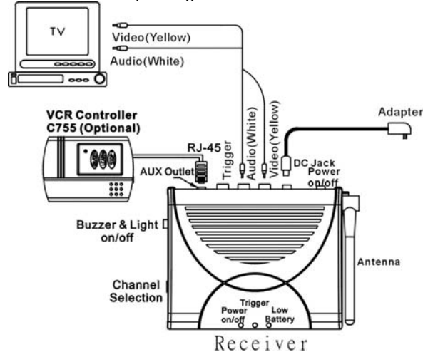
Figure 7 American Version
