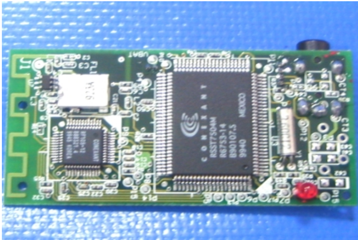
Component View of EUT FB004
