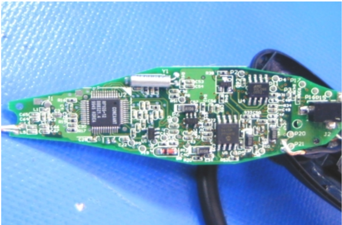
Solder View of EUT FE004
