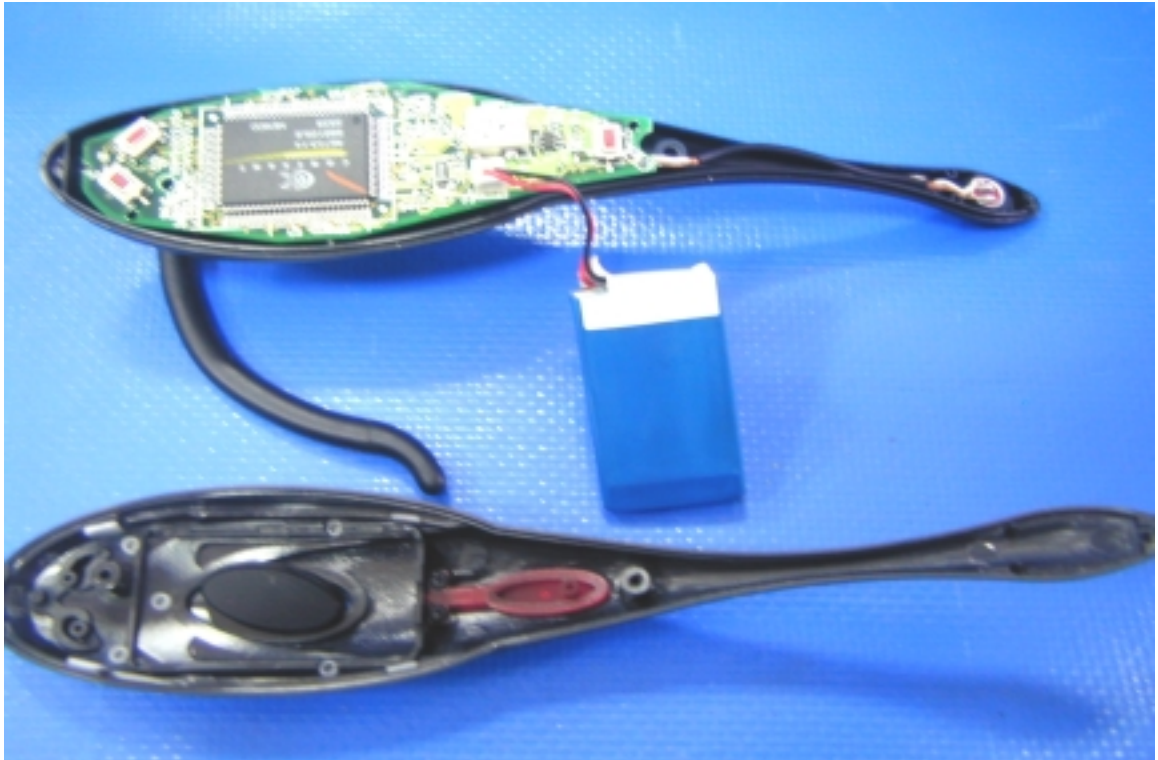
Inside View of EUT FE004
