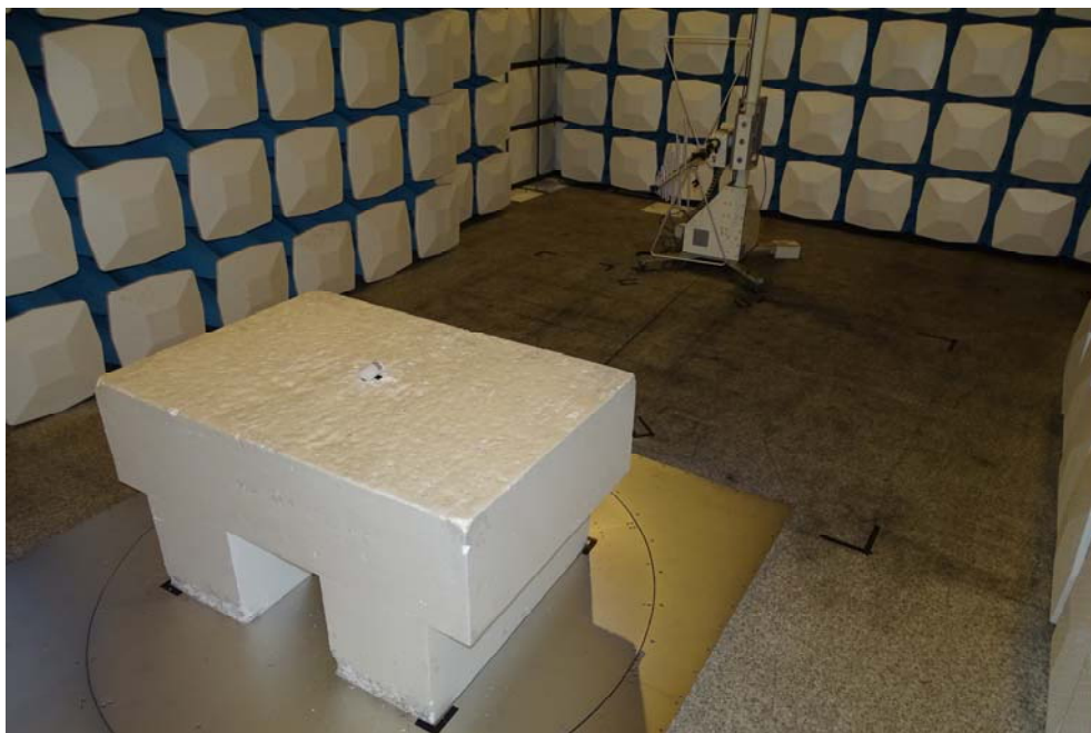
Back View of Radiated Test
