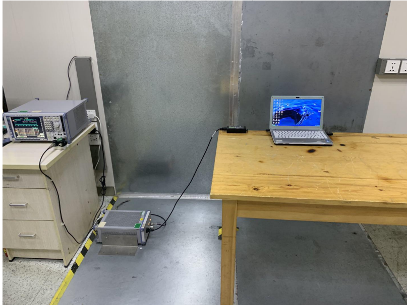
FCC ID: FU5SA370 Conducted Emissions
