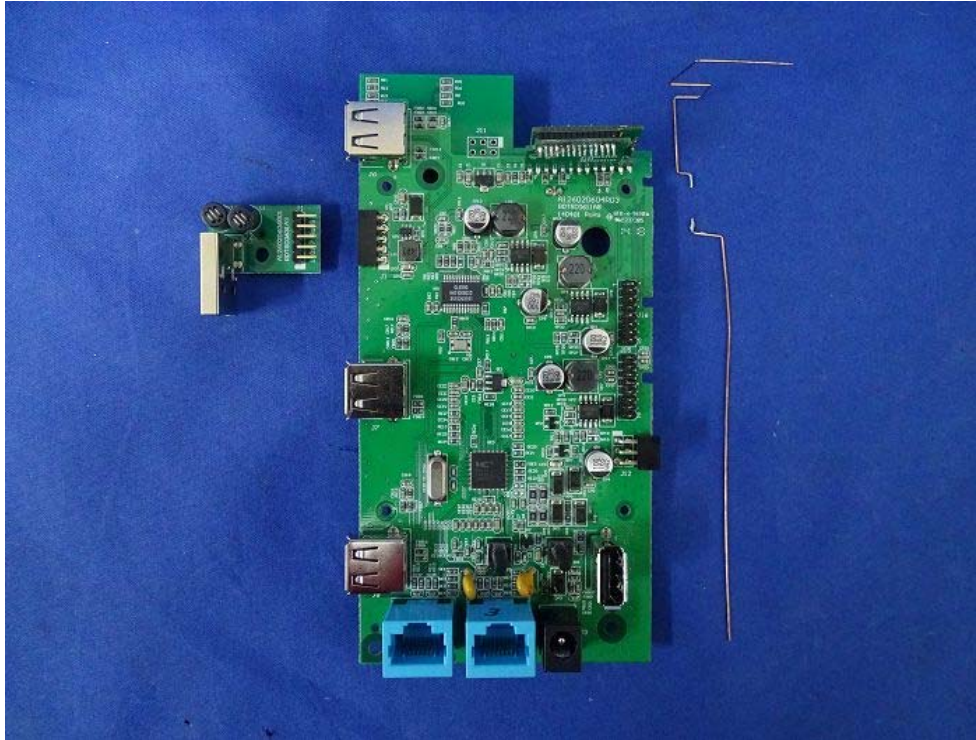
(25) EUT Photo
