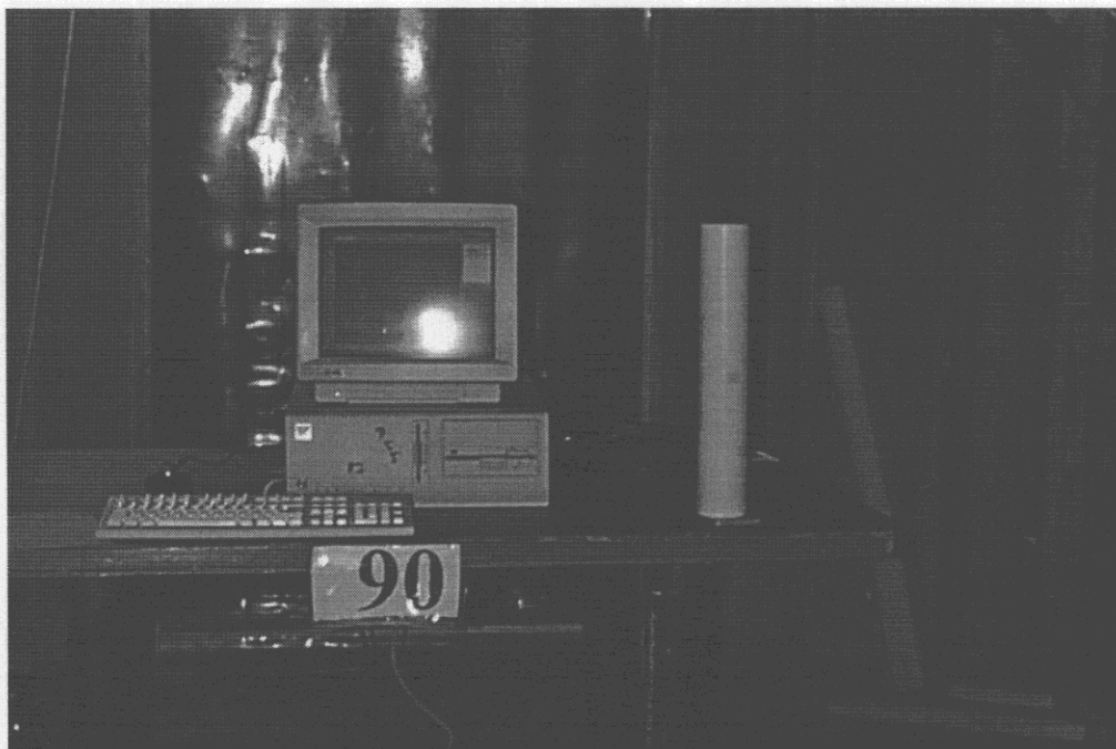
15.205 Restricted Band Test Setup Amp 13.5 dBi YAGI Antenna
