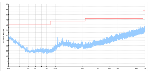
Figure 8.1-8: Radiated disturbance spectral plot (30 to 1000 MHz), Scanning at middle frequency, SRX1200-D
