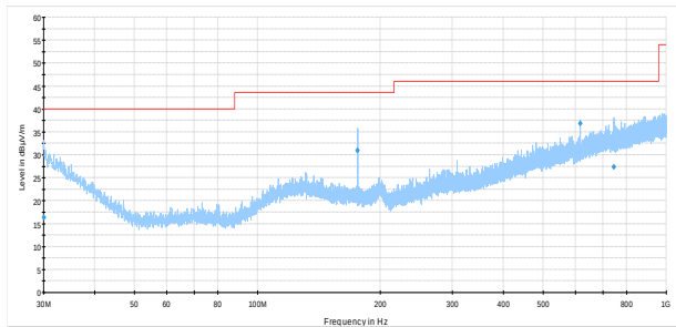
Figure 8.1-7: Radiated disturbance spectral plot (30 to 1000 MHz), Scanning at low frequency, SRX1200-D
