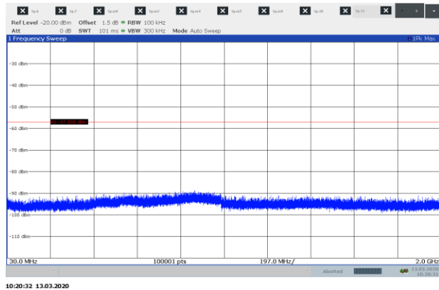
Figure 8.1-27: Receiver antenna power conducted emission spectral plot (30 to 2000 MHz), Scanning at high frequency, SRX1200
