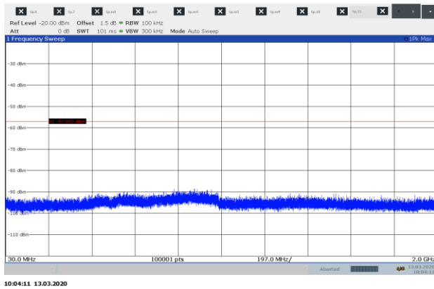
Figure 8.1-25: Receiver antenna power conducted emission spectral plot (30 to 2000 MHz), Scanning at low frequency, SRX1200
