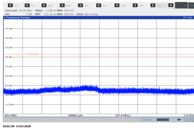
Figure 8.1-29: Receiver antenna power conducted emission spectral plot (30 to 2000 MHz), Scanning stopped at middle frequency, SRX1200
