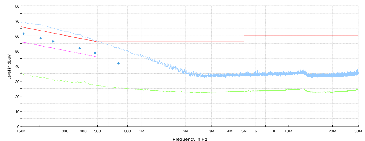
Figure 8.2-1: Conducted emissions – from AC mains power ports spectral plot on phase line (SRX1200)
