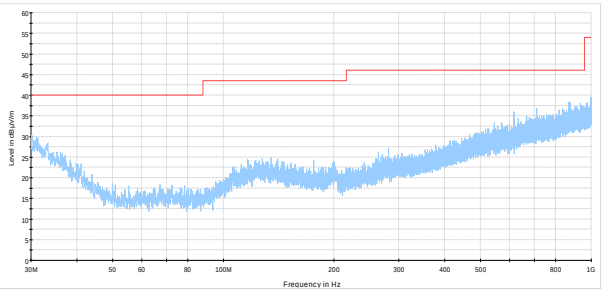
Figure 8.1-9: Radiated disturbance spectral plot (30 to 1000 MHz), Scanning at high frequency, SRX1200-D
