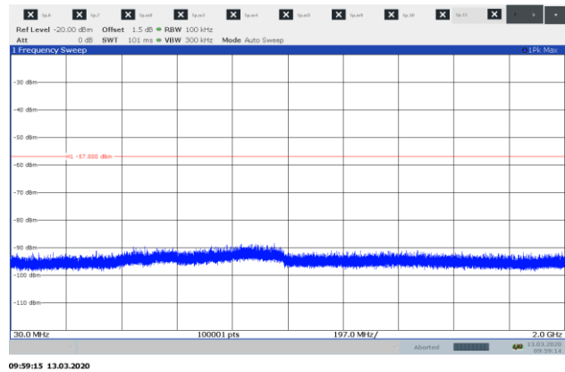
Figure 8.1-26: Receiver antenna power conducted emission spectral plot (30 to 2000 MHz), Scanning at middle frequency, SRX1200
