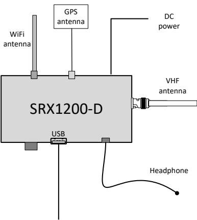
Figure 3.5-1: Setup diagram
