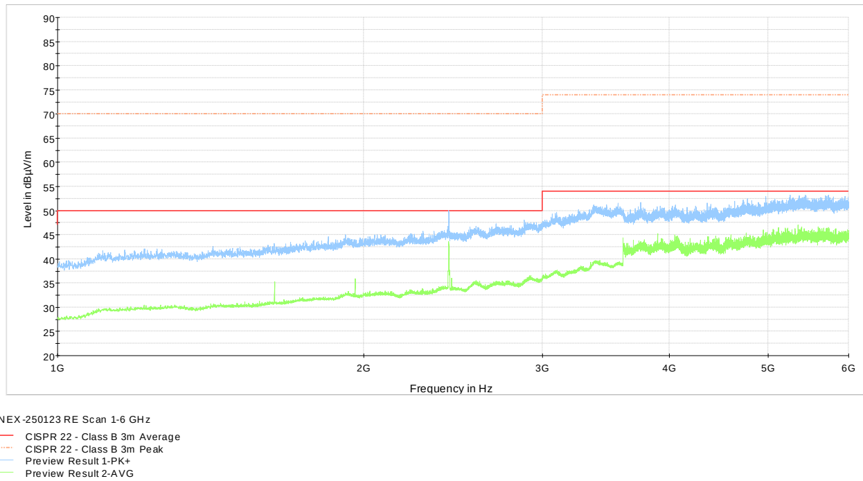
Figure 8.1-2: Radiated disturbance spectral plot (1 to 6 GHz)
