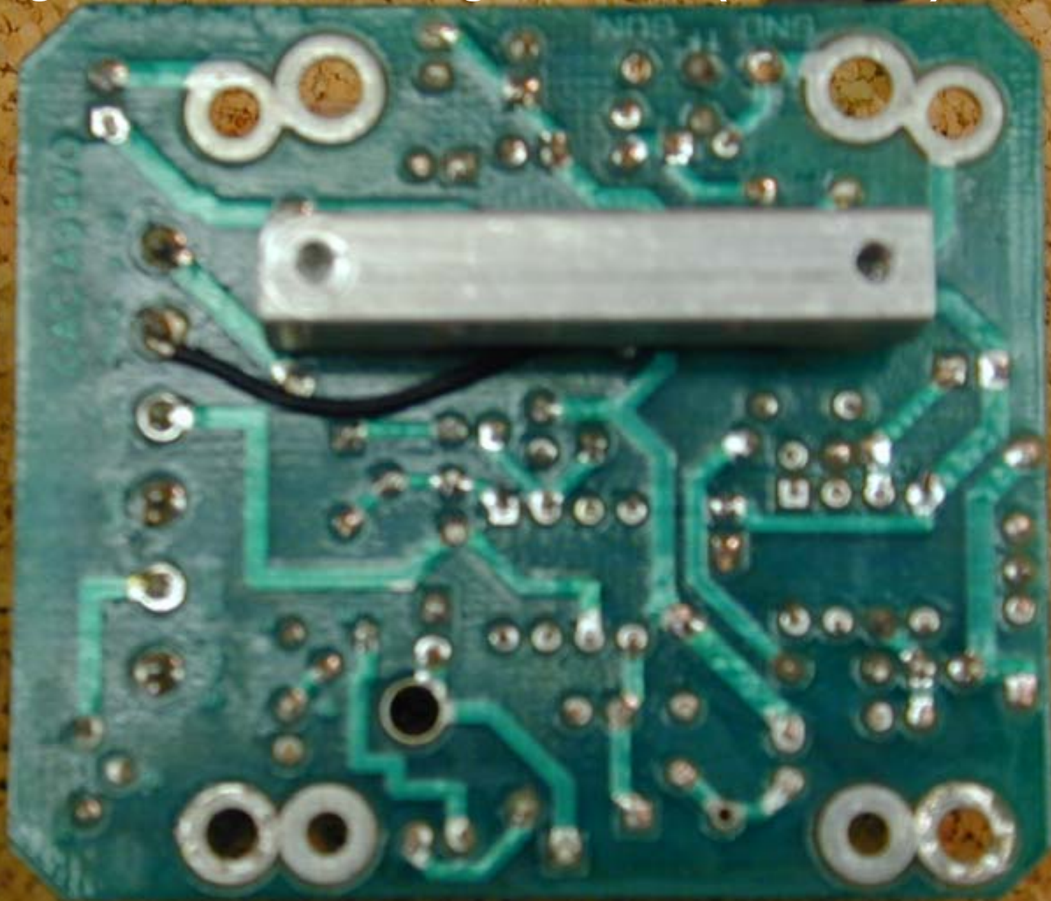
PCB Signal Processing Board (bottom)
