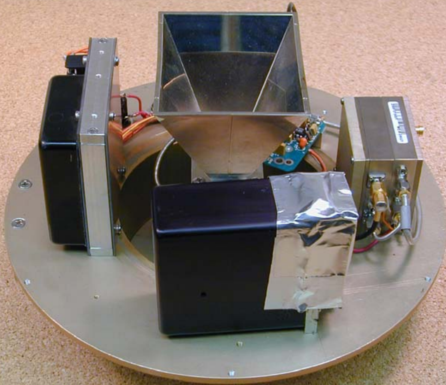
DUT with Radome Removed (side 3)
