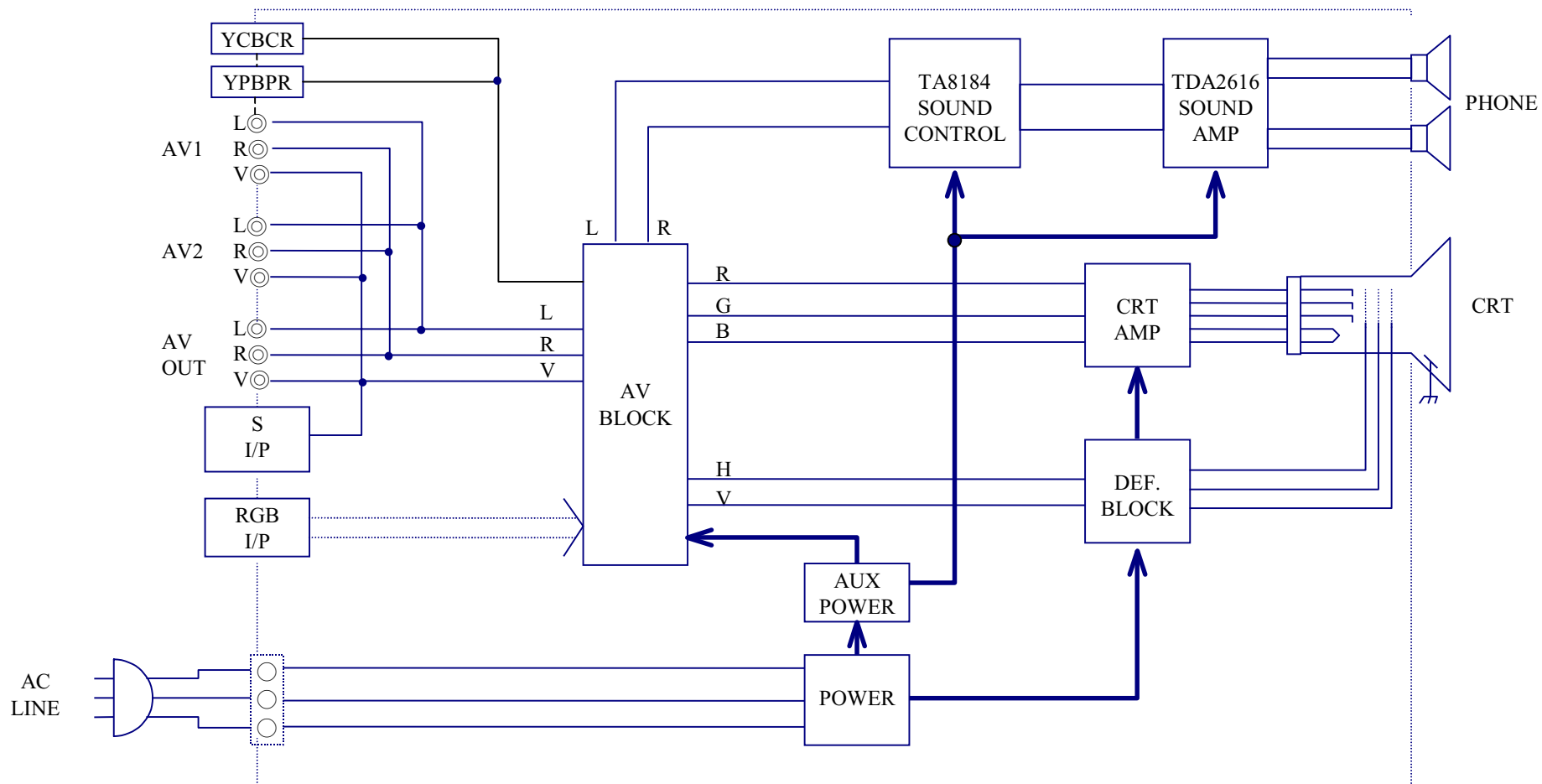
Total block diagram
