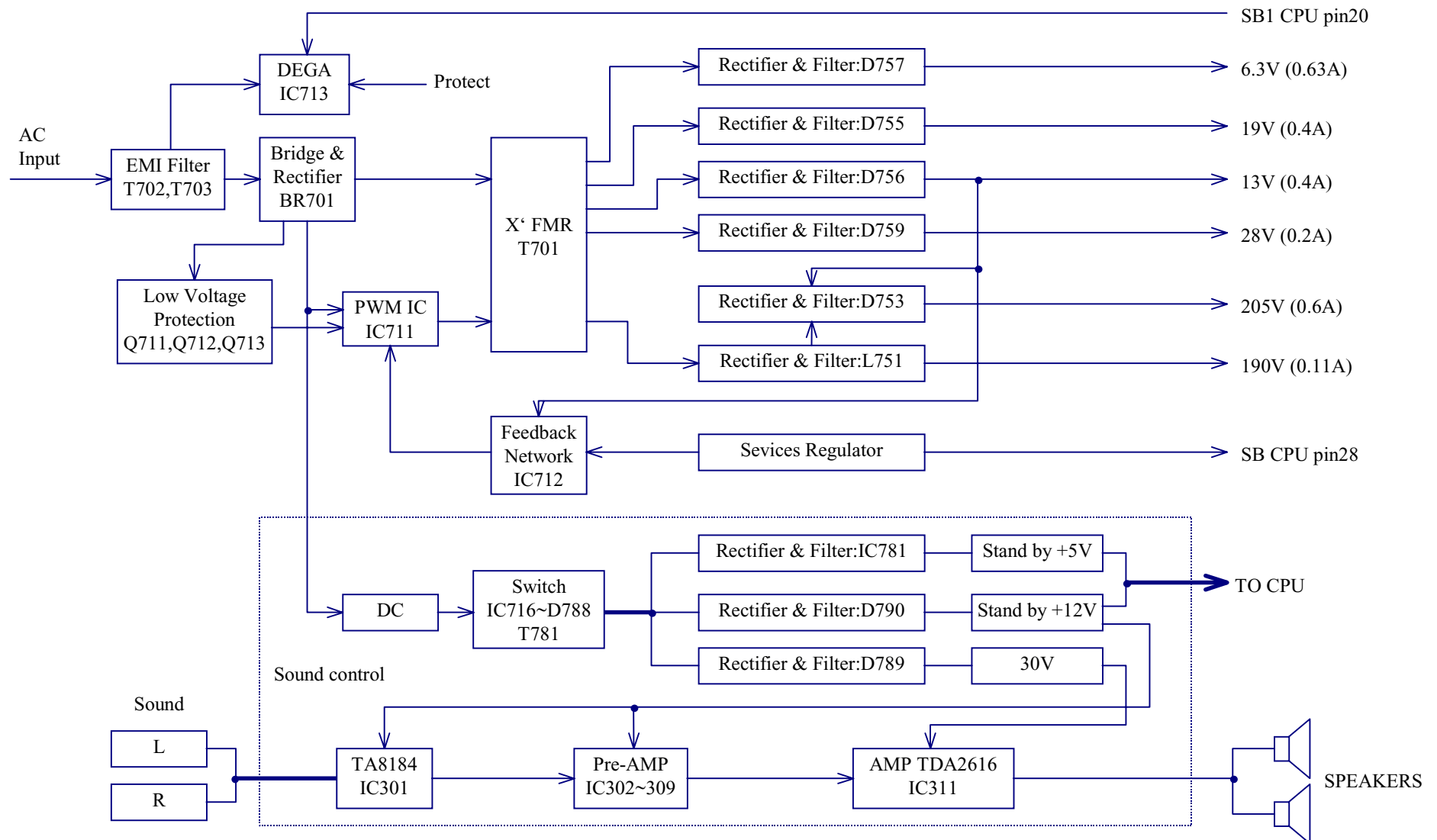
Main power supply &amp; Aux. power &amp; sound AMP block diagram
