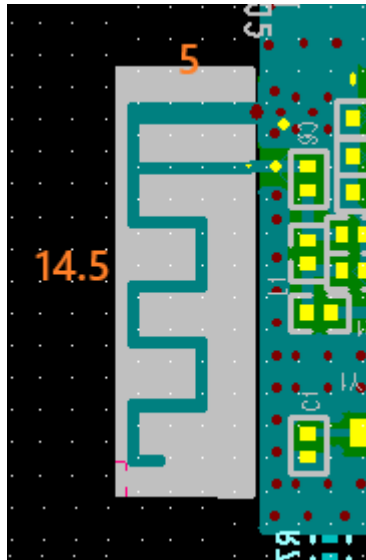
Figure 1 Physical dimension (mm)
