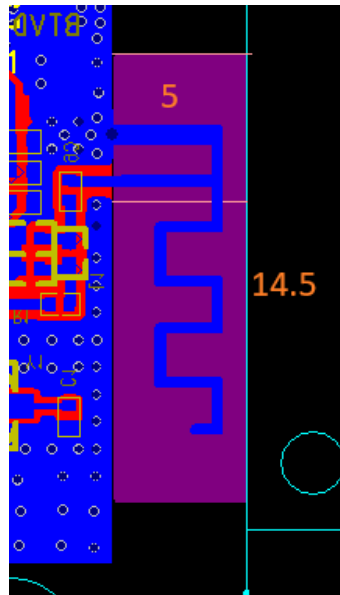
Figure 1 Physical dimension (mm)
