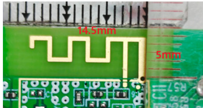
Figure 1 Physical dimension (mm)
