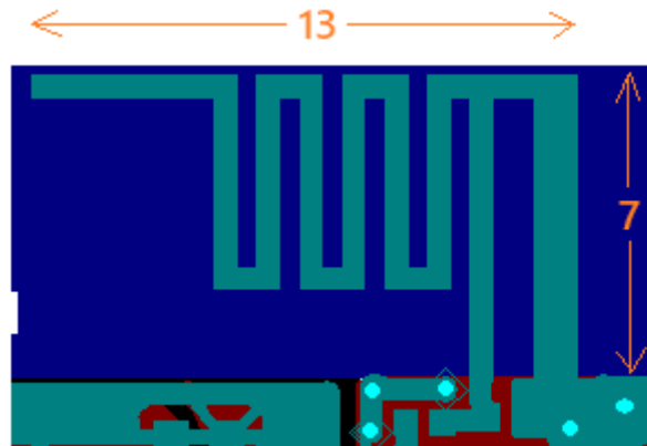
Figure 1 Physical dimension (mm)
