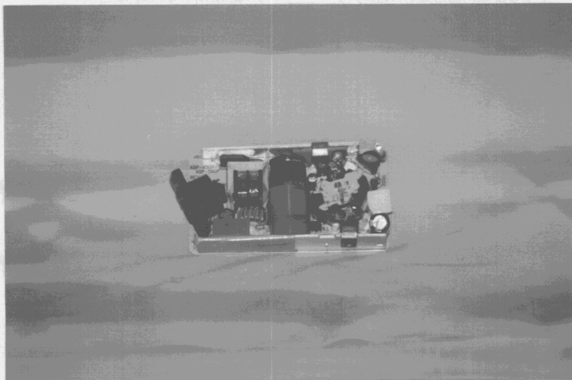
Adaptor Main Board Component Side View
