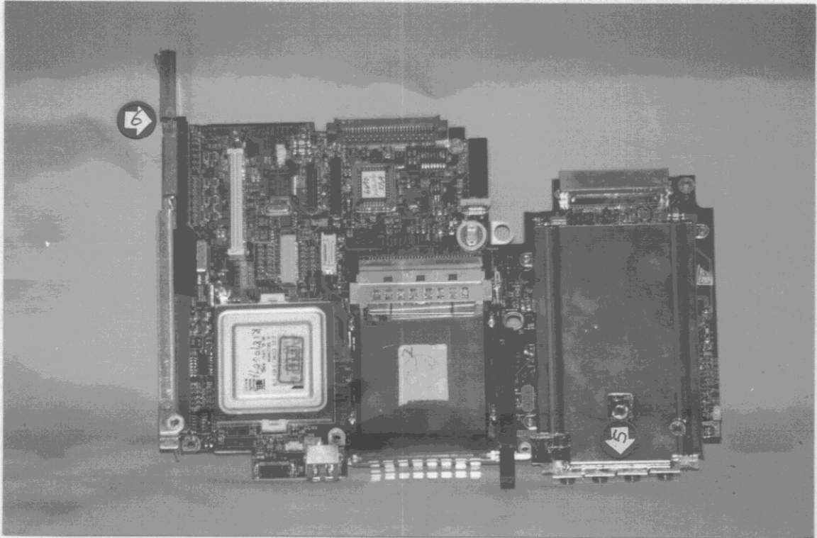
Mother Board with Gasket and Spring Finger Top View
