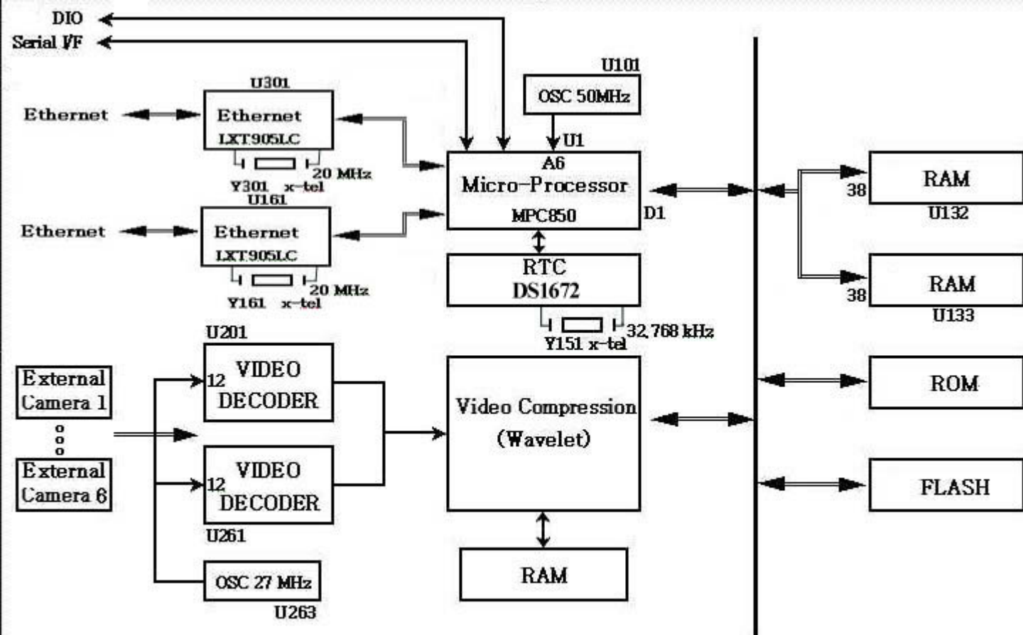
NetServer-6 Block Diagram
