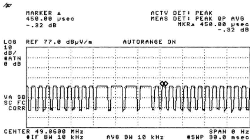
Figure C [Short Pulse]
