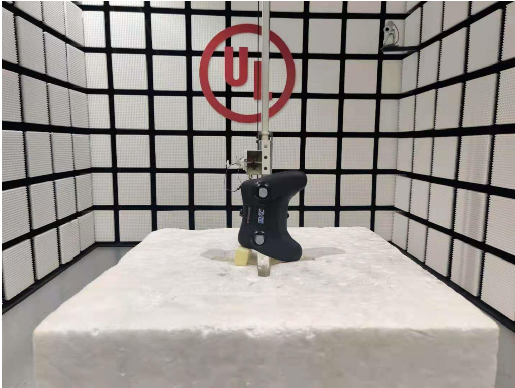
Radiated Disturbance Setup (Above 1 GHz – Z axis)
