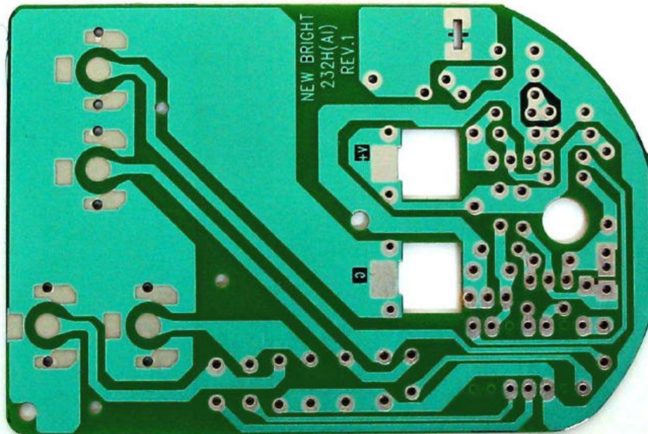
Model : 2322H(49M) Soldering side
