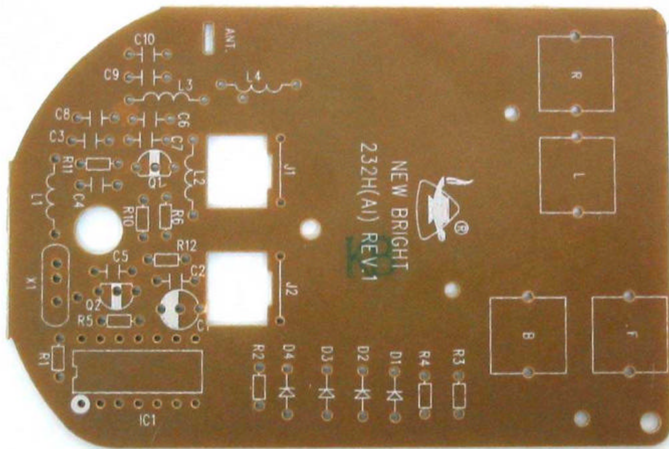
Model : 2322H(49M) Component side
