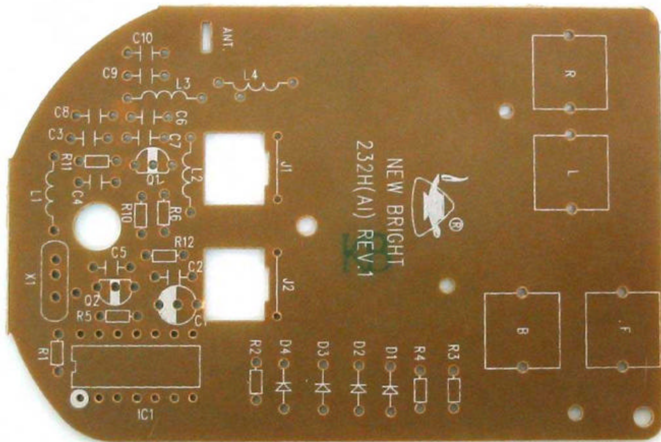
Model : 232H (27M) Component side
