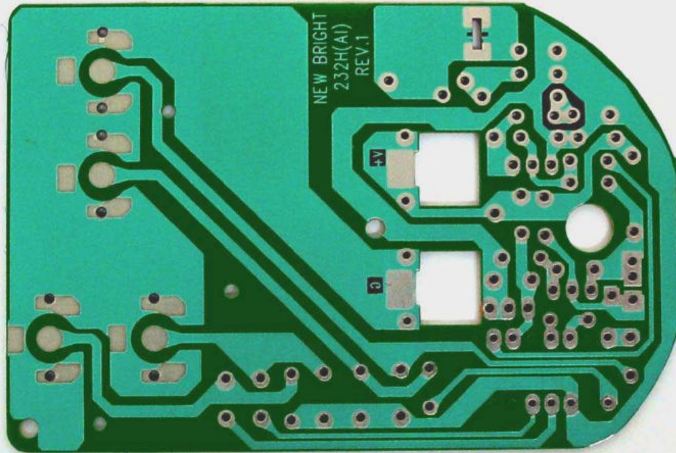
Model : 232H (27M) Soldering side
