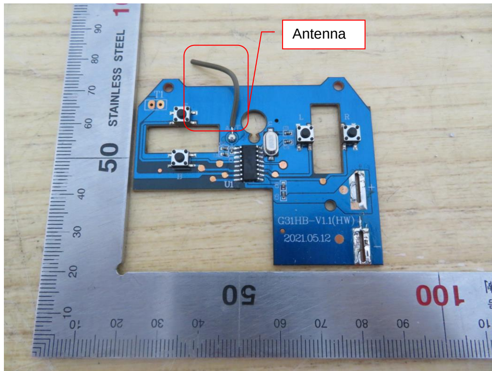
Internal View of EUT (Version 3)-4
