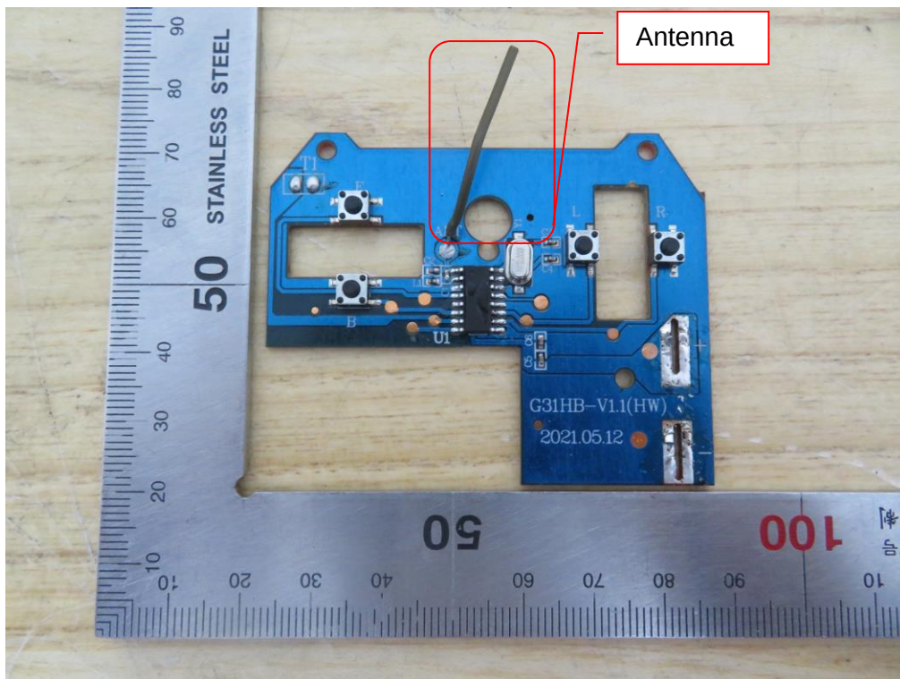
Internal View of EUT (Version 1)-4
