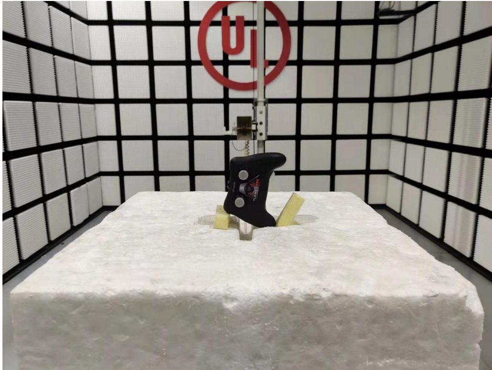
Radiated Disturbance Setup (Above 1 GHz – Z axis)
