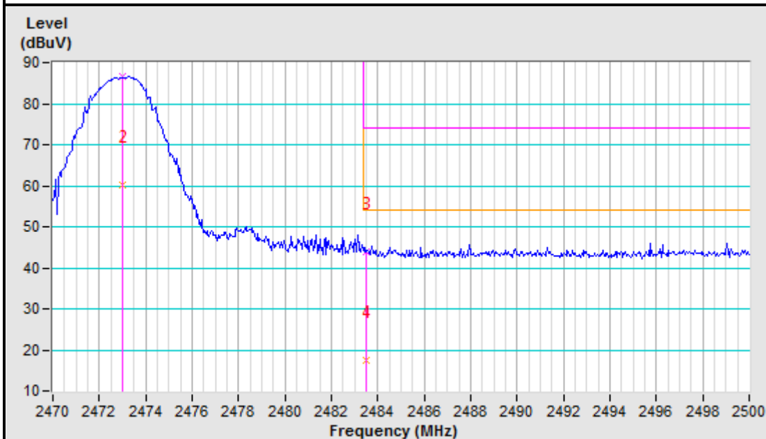
2473MHz Vertical
