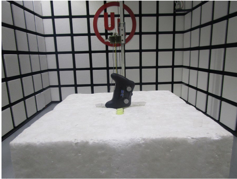
Radiated Disturbance Setup (Above 1 GHz – Y axis)
