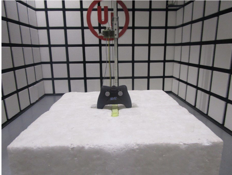
Radiated Disturbance Setup (Above 1 GHz – Z axis)
